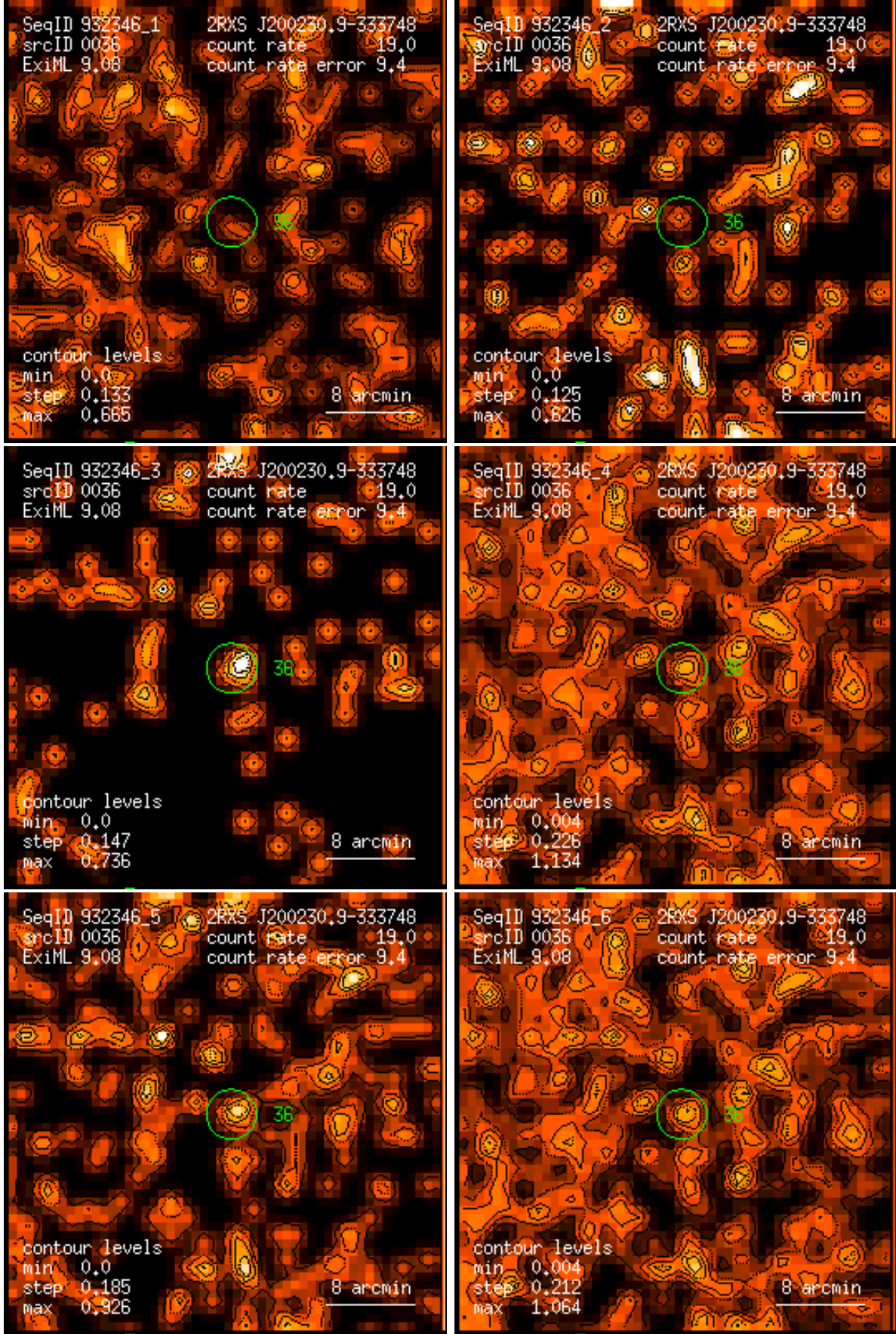
Figure 36: RASS 932346: detection 0036: band rate images, Gaussian filter: (1) PSPC channels 11 – 41, (2) 52 – 90, (3) 91 – 201, (4) 11 – 235, (5) 52 – 201, (6) 11 – 201. Broad band rates in counts/ks. Band rate contour levels in counts/ks/arcmin 2 .
