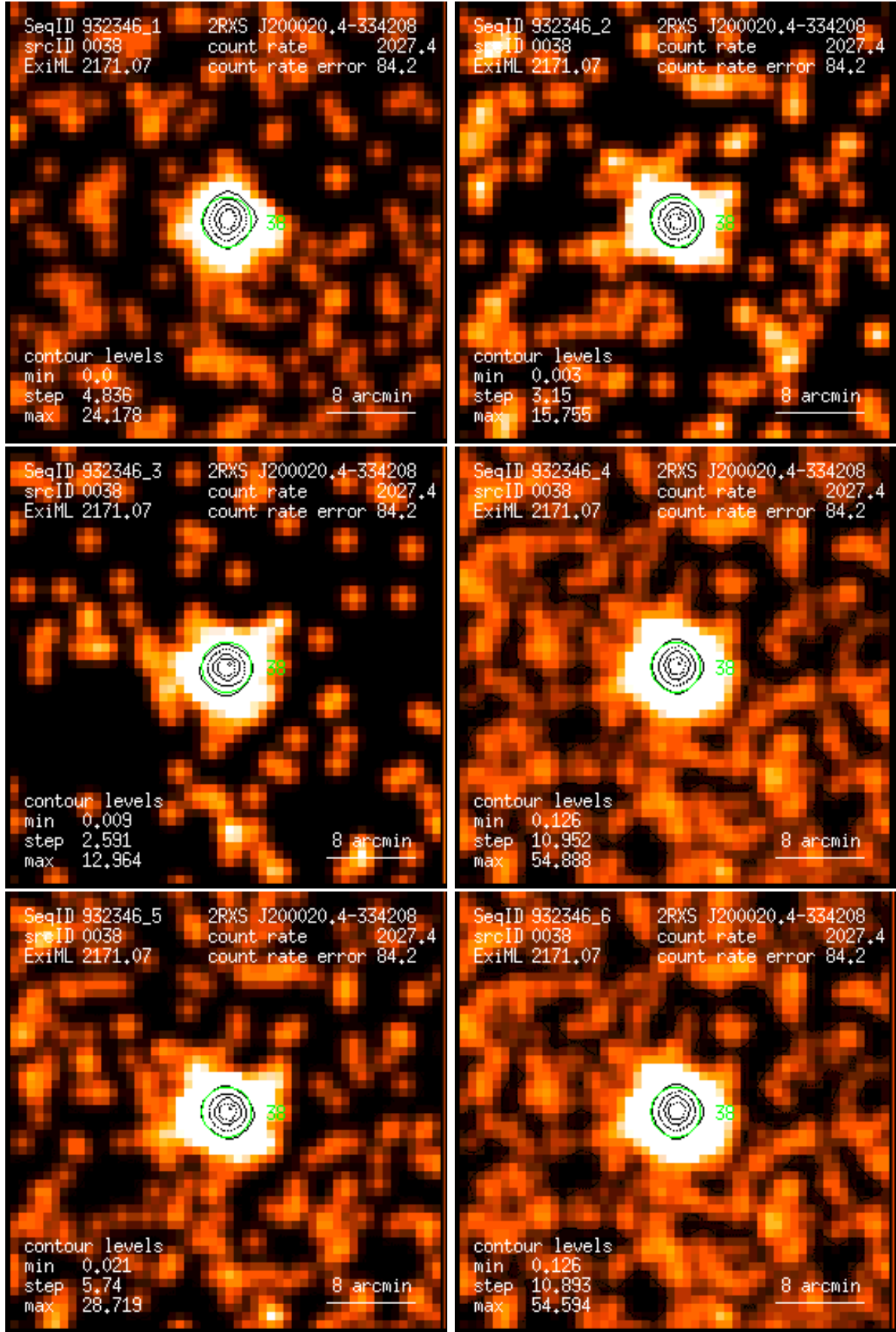
Figure 38: RASS 932346: detection 0038: band rate images, Gaussian filter: (1) PSPC channels 11 – 41, (2) 52 – 90, (3) 91 – 201, (4) 11 – 235, (5) 52 – 201, (6) 11 – 201. Broad band rates in counts/ks. Band rate contour levels in counts/ks/arcmin 2 .
