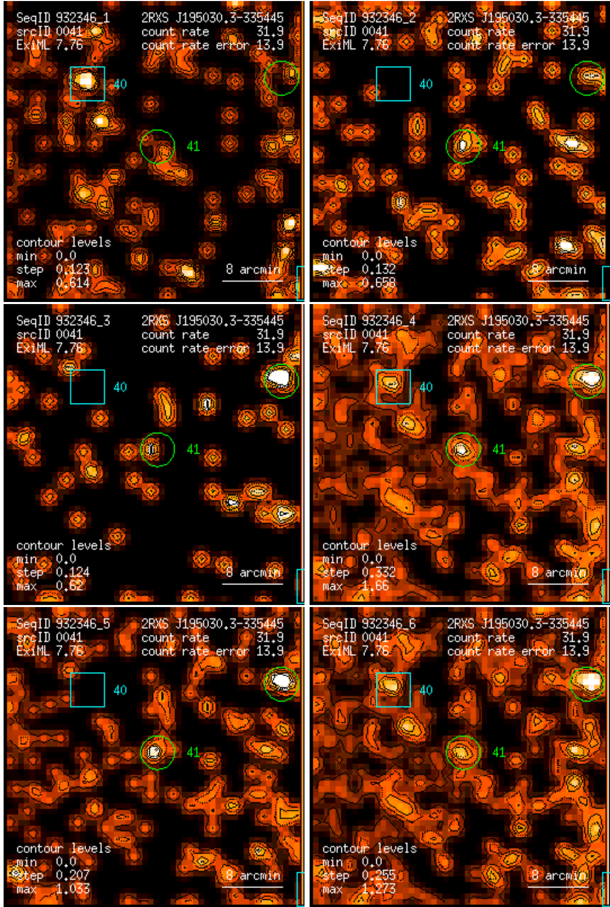
Figure 41: RASS 932346: detection 0041: band rate images, Gaussian filter: (1) PSPC channels 11 – 41, (2) 52 – 90, (3) 91 – 201, (4) 11 – 235, (5) 52 – 201, (6) 11 – 201. Broad band rates in counts/ks. Band rate contour levels in counts/ks/arcmin 2 .
