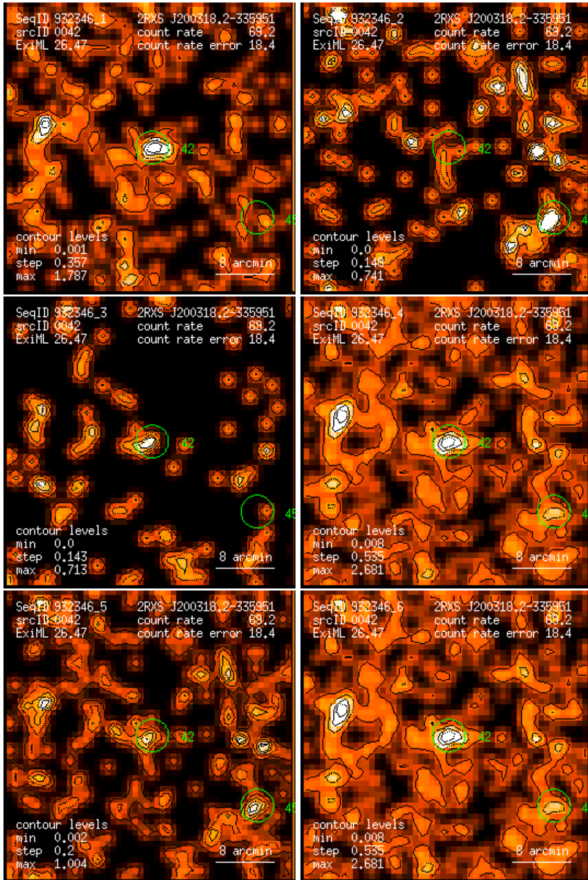
Figure 42: RASS 932346: detection 0042: band rate images, Gaussian filter: (1) PSPC channels 11 – 41, (2) 52 – 90, (3) 91 – 201, (4) 11 – 235, (5) 52 – 201, (6) 11 – 201. Broad band rates in counts/ks. Band rate contour levels in counts/ks/arcmin 2 .
