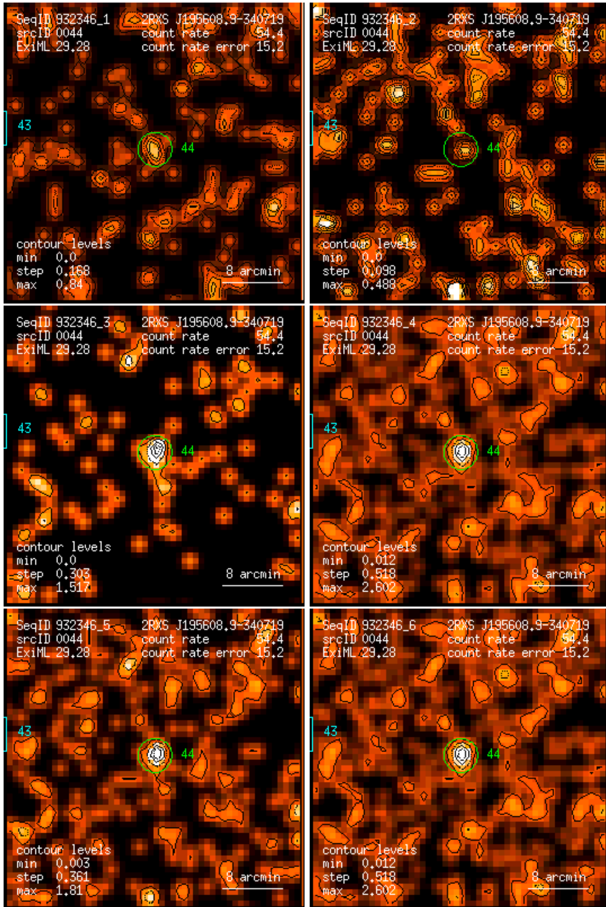
Figure 44: RASS 932346: detection 0044: band rate images, Gaussian filter: (1) PSPC channels 11 – 41, (2) 52 – 90, (3) 91 – 201, (4) 11 – 235, (5) 52 – 201, (6) 11 – 201. Broad band rates in counts/ks. Band rate contour levels in counts/ks/arcmin 2 .
