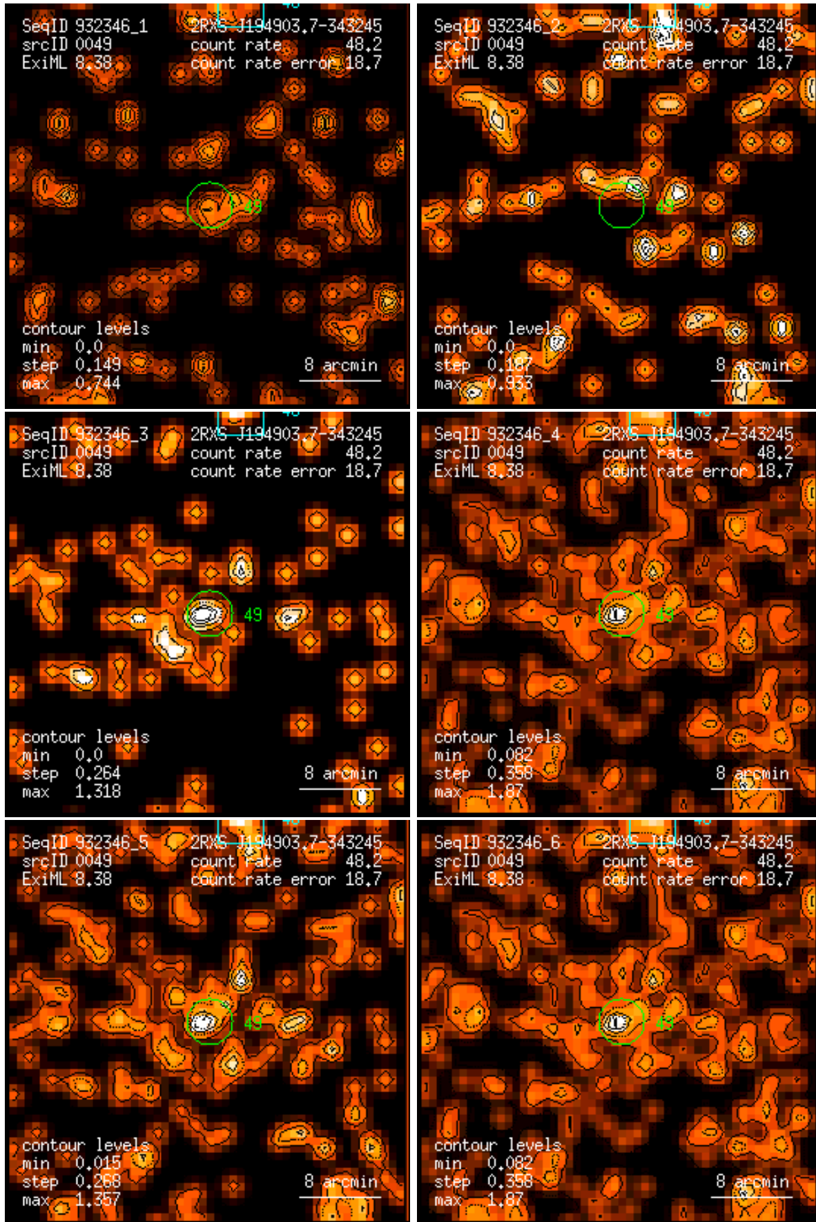
Figure 49: RASS 932346: detection 0049: band rate images, Gaussian filter: (1) PSPC channels 11 – 41, (2) 52 – 90, (3) 91 – 201, (4) 11 – 235, (5) 52 – 201, (6) 11 – 201. Broad band rates in counts/ks. Band rate contour levels in counts/ks/arcmin 2 .
