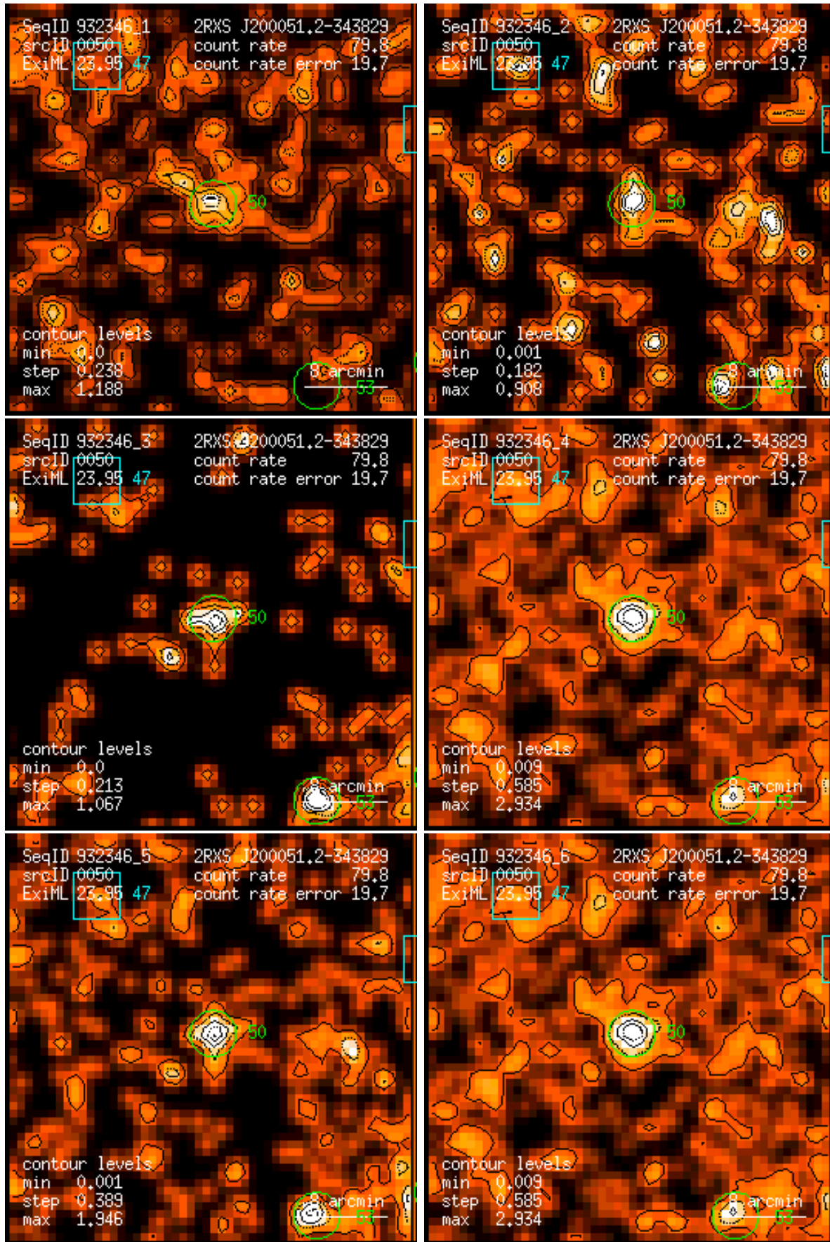
Figure 50: RASS 932346: detection 0050: band rate images, Gaussian filter: (1) PSPC channels 11 – 41, (2) 52 – 90, (3) 91 – 201, (4) 11 – 235, (5) 52 – 201, (6) 11 – 201. Broad band rates in counts/ks. Band rate contour levels in counts/ks/arcmin 2 .
