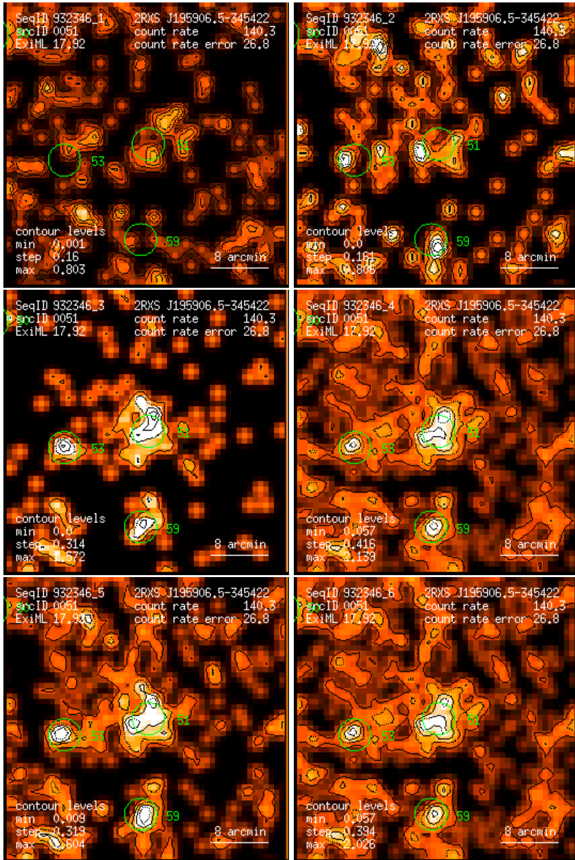
Figure 51: RASS 932346: detection 0051: band rate images, Gaussian filter: (1) PSPC channels 11 – 41, (2) 52 – 90, (3) 91 – 201, (4) 11 – 235, (5) 52 – 201, (6) 11 – 201. Broad band rates in counts/ks. Band rate contour levels in counts/ks/arcmin 2 .
