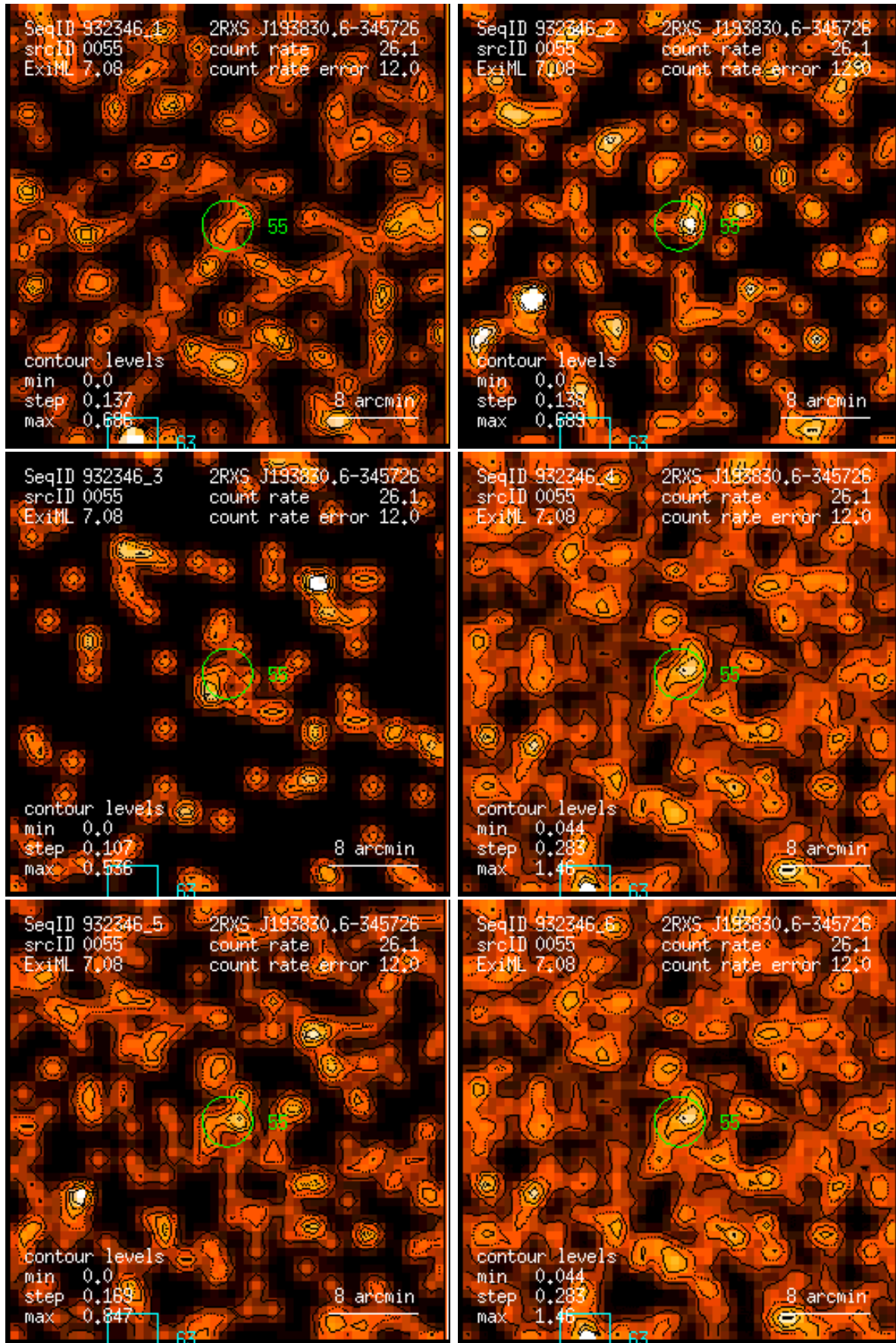
Figure 55: RASS 932346: detection 0055: band rate images, Gaussian filter: (1) PSPC channels 11 – 41, (2) 52 – 90, (3) 91 – 201, (4) 11 – 235, (5) 52 – 201, (6) 11 – 201. Broad band rates in counts/ks. Band rate contour levels in counts/ks/arcmin 2 .
