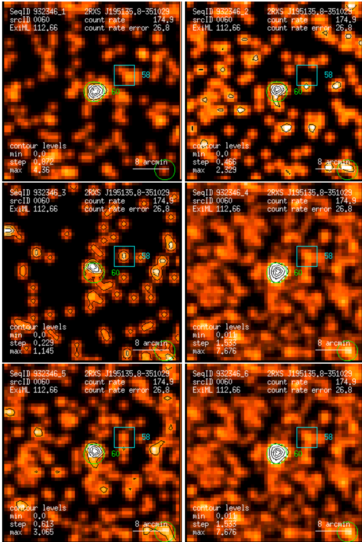
Figure 60: RASS 932346: detection 0060: band rate images, Gaussian filter: (1) PSPC channels 11 – 41, (2) 52 – 90, (3) 91 – 201, (4) 11 – 235, (5) 52 – 201, (6) 11 – 201. Broad band rates in counts/ks. Band rate contour levels in counts/ks/arcmin 2 .
