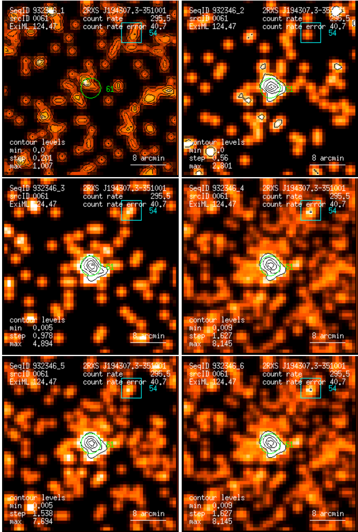
Figure 61: RASS 932346: detection 0061: band rate images, Gaussian filter: (1) PSPC channels 11 – 41, (2) 52 – 90, (3) 91 – 201, (4) 11 – 235, (5) 52 – 201, (6) 11 – 201. Broad band rates in counts/ks. Band rate contour levels in counts/ks/arcmin 2 .
