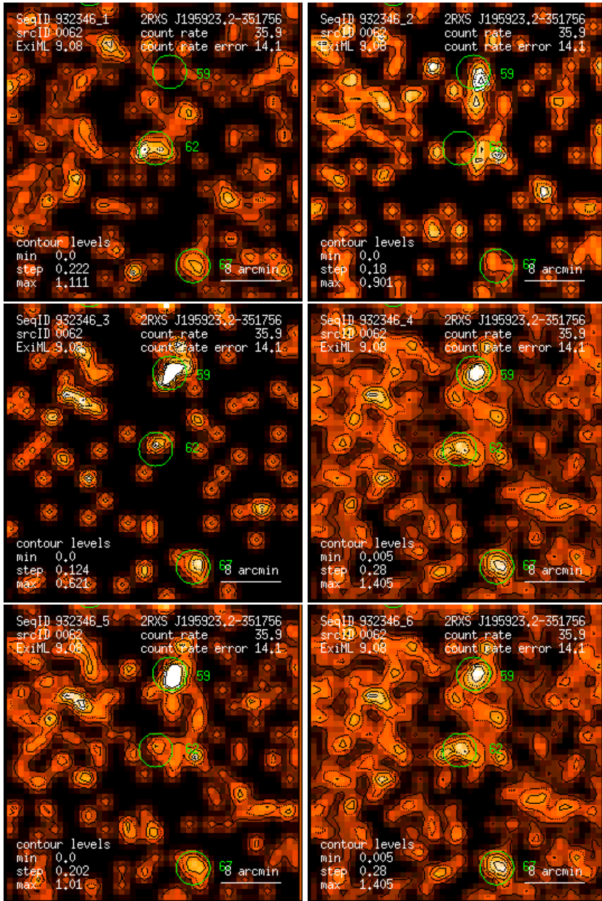
Figure 62: RASS 932346: detection 0062: band rate images, Gaussian filter: (1) PSPC channels 11 – 41, (2) 52 – 90, (3) 91 – 201, (4) 11 – 235, (5) 52 – 201, (6) 11 – 201. Broad band rates in counts/ks. Band rate contour levels in counts/ks/arcmin 2 .
