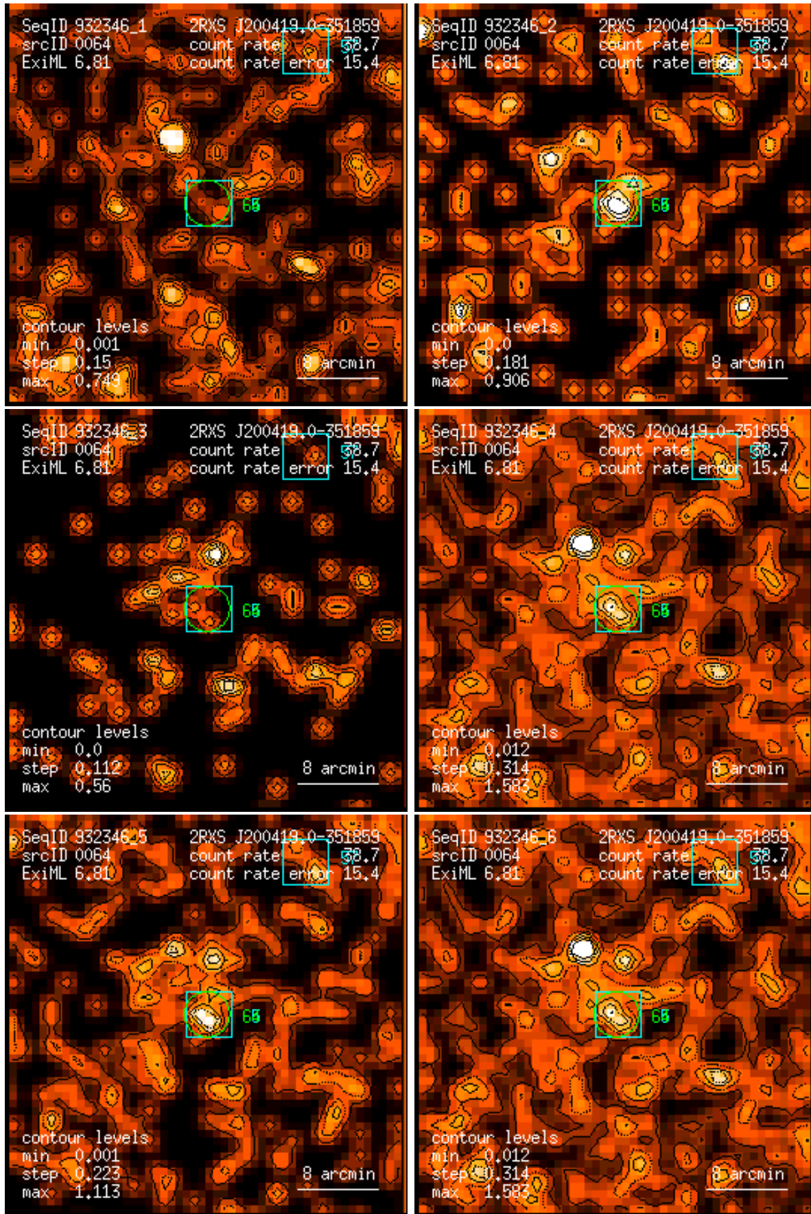
Figure 64: RASS 932346: detection 0064: band rate images, Gaussian filter: (1) PSPC channels 11 – 41, (2) 52 – 90, (3) 91 – 201, (4) 11 – 235, (5) 52 – 201, (6) 11 – 201. Broad band rates in counts/ks. Band rate contour levels in counts/ks/arcmin 2 .
