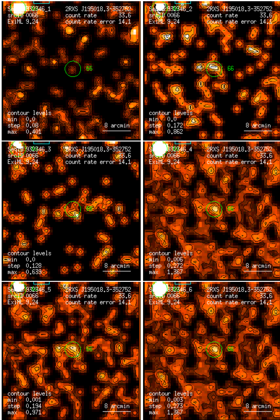
Figure 66: RASS 932346: detection 0066: band rate images, Gaussian filter: (1) PSPC channels 11 – 41, (2) 52 – 90, (3) 91 – 201, (4) 11 – 235, (5) 52 – 201, (6) 11 – 201. Broad band rates in counts/ks. Band rate contour levels in counts/ks/arcmin 2 .
