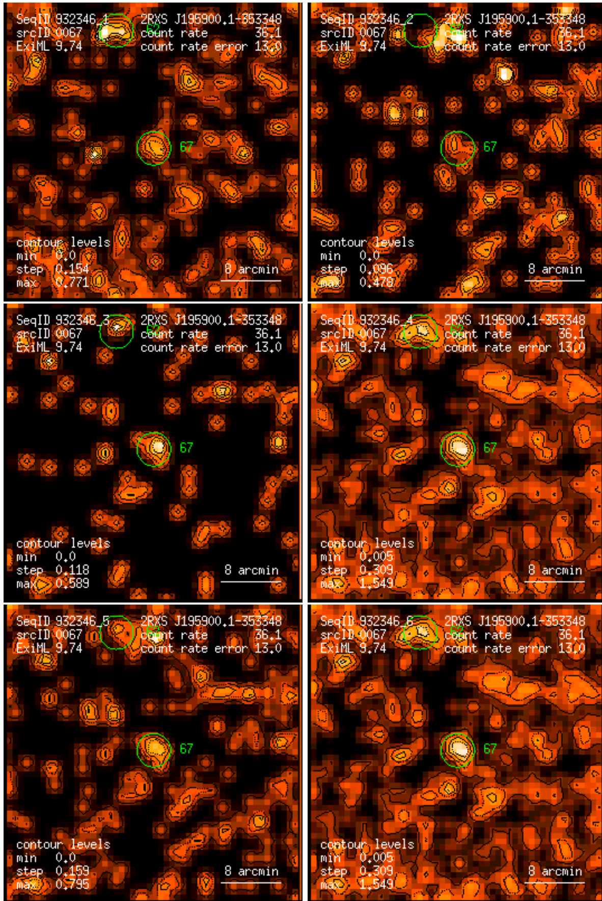
Figure 67: RASS 932346: detection 0067: band rate images, Gaussian filter: (1) PSPC channels 11 – 41, (2) 52 – 90, (3) 91 – 201, (4) 11 – 235, (5) 52 – 201, (6) 11 – 201. Broad band rates in counts/ks. Band rate contour levels in counts/ks/arcmin 2 .
