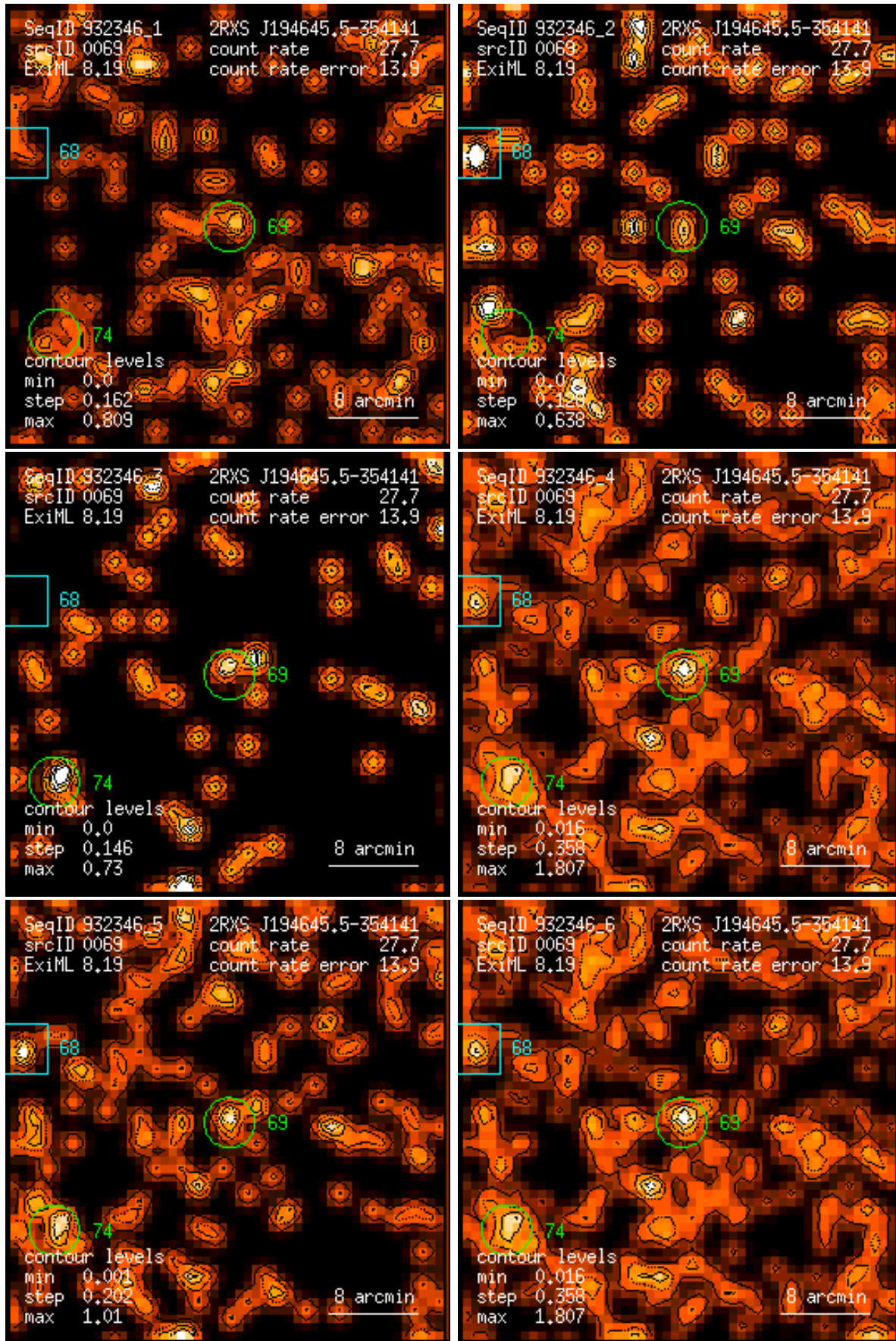
Figure 69: RASS 932346: detection 0069: band rate images, Gaussian filter: (1) PSPC channels 11 – 41, (2) 52 – 90, (3) 91 – 201, (4) 11 – 235, (5) 52 – 201, (6) 11 – 201. Broad band rates in counts/ks. Band rate contour levels in counts/ks/arcmin 2 .
