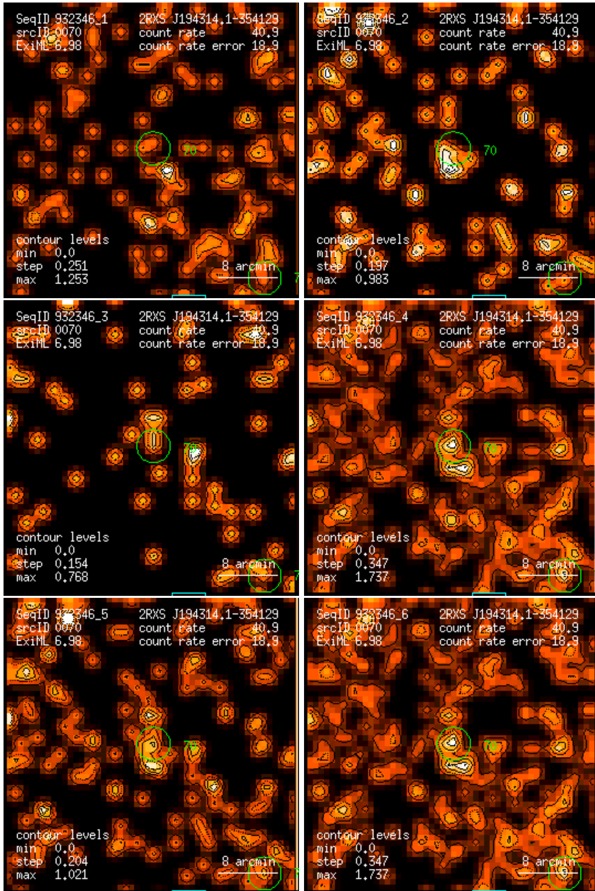
Figure 70: RASS 932346: detection 0070: band rate images, Gaussian filter: (1) PSPC channels 11 – 41, (2) 52 – 90, (3) 91 – 201, (4) 11 – 235, (5) 52 – 201, (6) 11 – 201. Broad band rates in counts/ks. Band rate contour levels in counts/ks/arcmin 2 .
