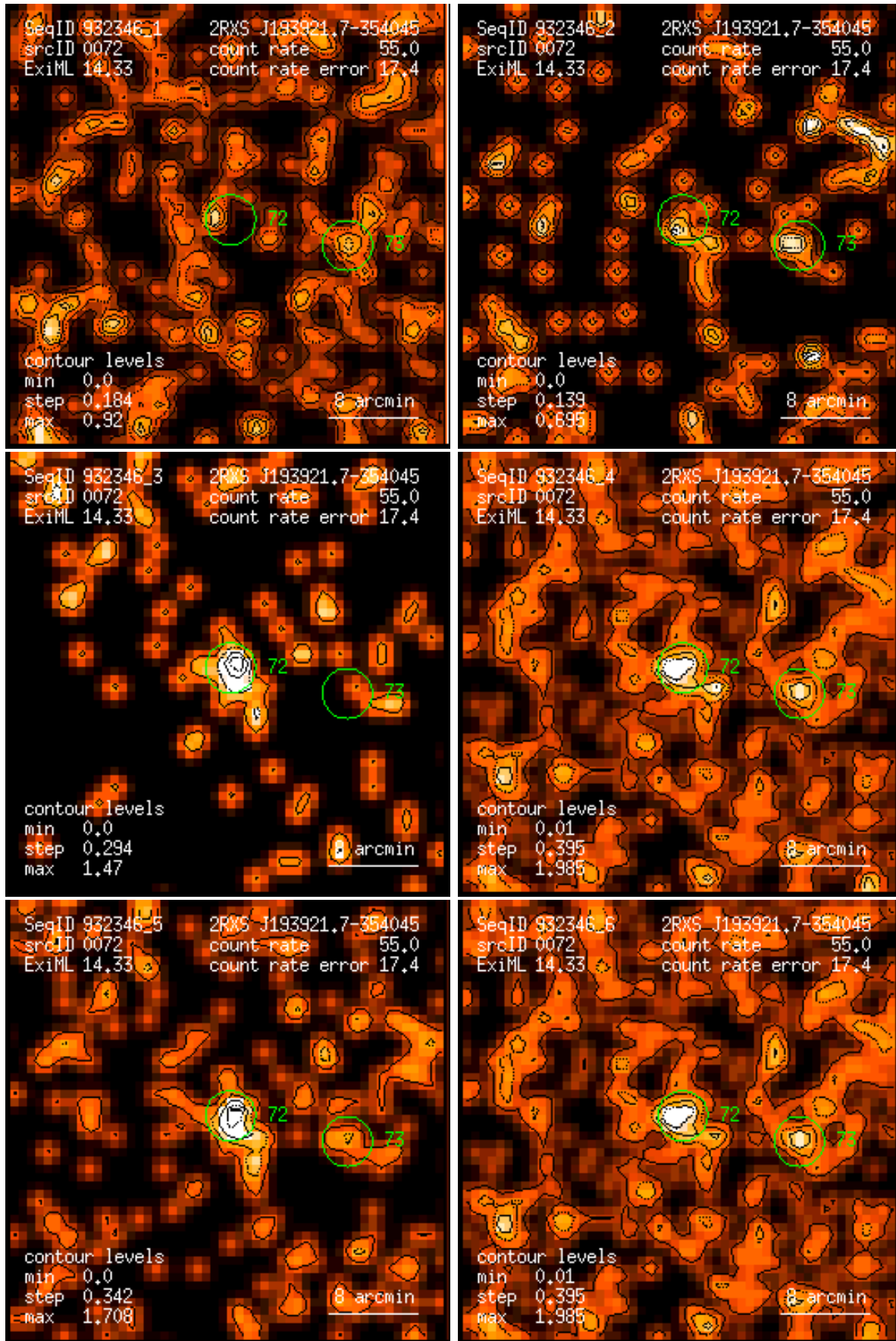
Figure 72: RASS 932346: detection 0072: band rate images, Gaussian filter: (1) PSPC channels 11 – 41, (2) 52 – 90, (3) 91 – 201, (4) 11 – 235, (5) 52 – 201, (6) 11 – 201. Broad band rates in counts/ks. Band rate contour levels in counts/ks/arcmin 2 .
