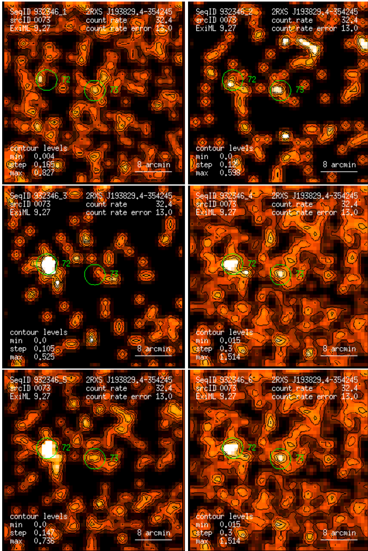
Figure 73: RASS 932346: detection 0073: band rate images, Gaussian filter: (1) PSPC channels 11 – 41, (2) 52 – 90, (3) 91 – 201, (4) 11 – 235, (5) 52 – 201, (6) 11 – 201. Broad band rates in counts/ks. Band rate contour levels in counts/ks/arcmin 2 .
