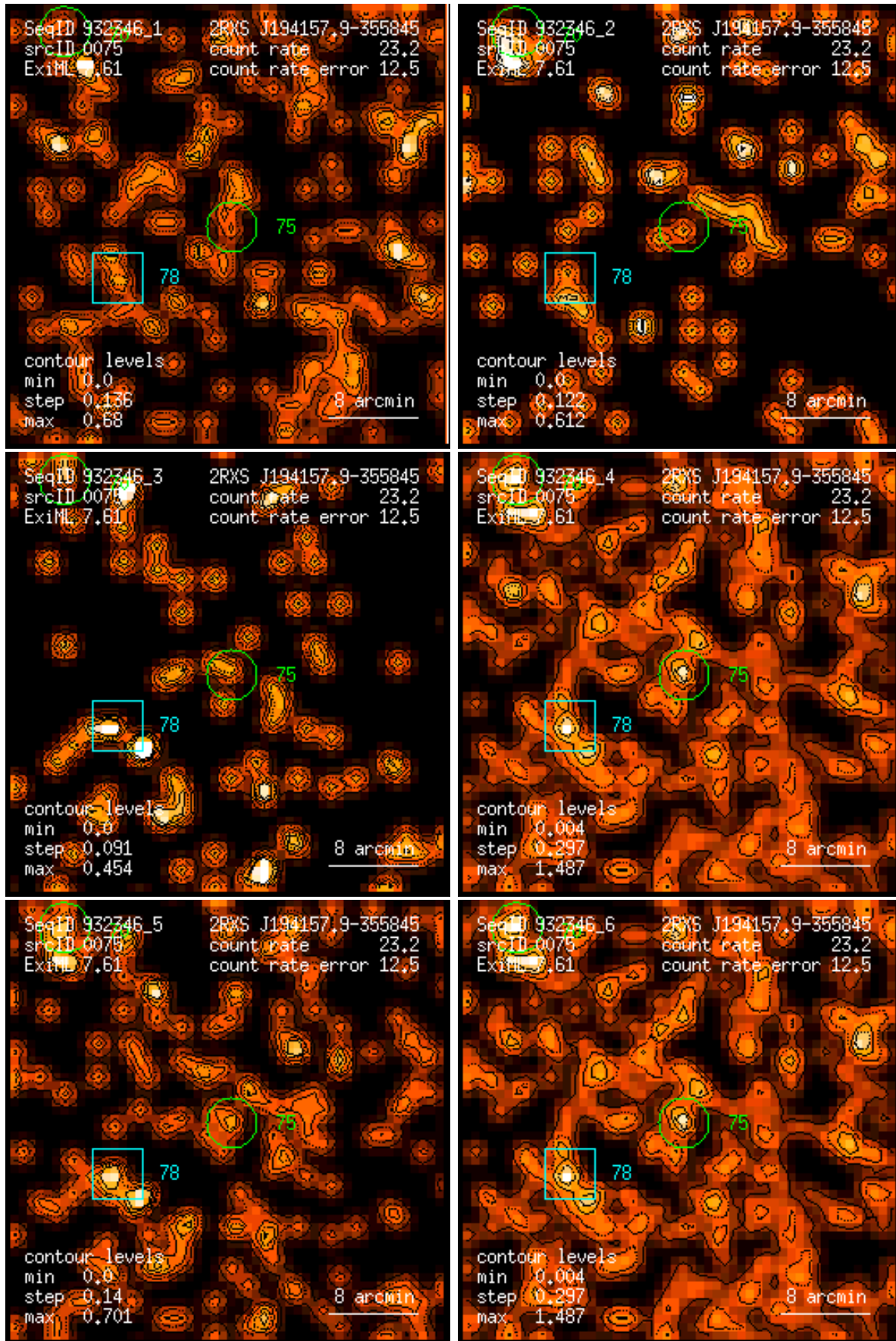
Figure 75: RASS 932346: detection 0075: band rate images, Gaussian filter: (1) PSPC channels 11 – 41, (2) 52 – 90, (3) 91 – 201, (4) 11 – 235, (5) 52 – 201, (6) 11 – 201. Broad band rates in counts/ks. Band rate contour levels in counts/ks/arcmin 2 .
