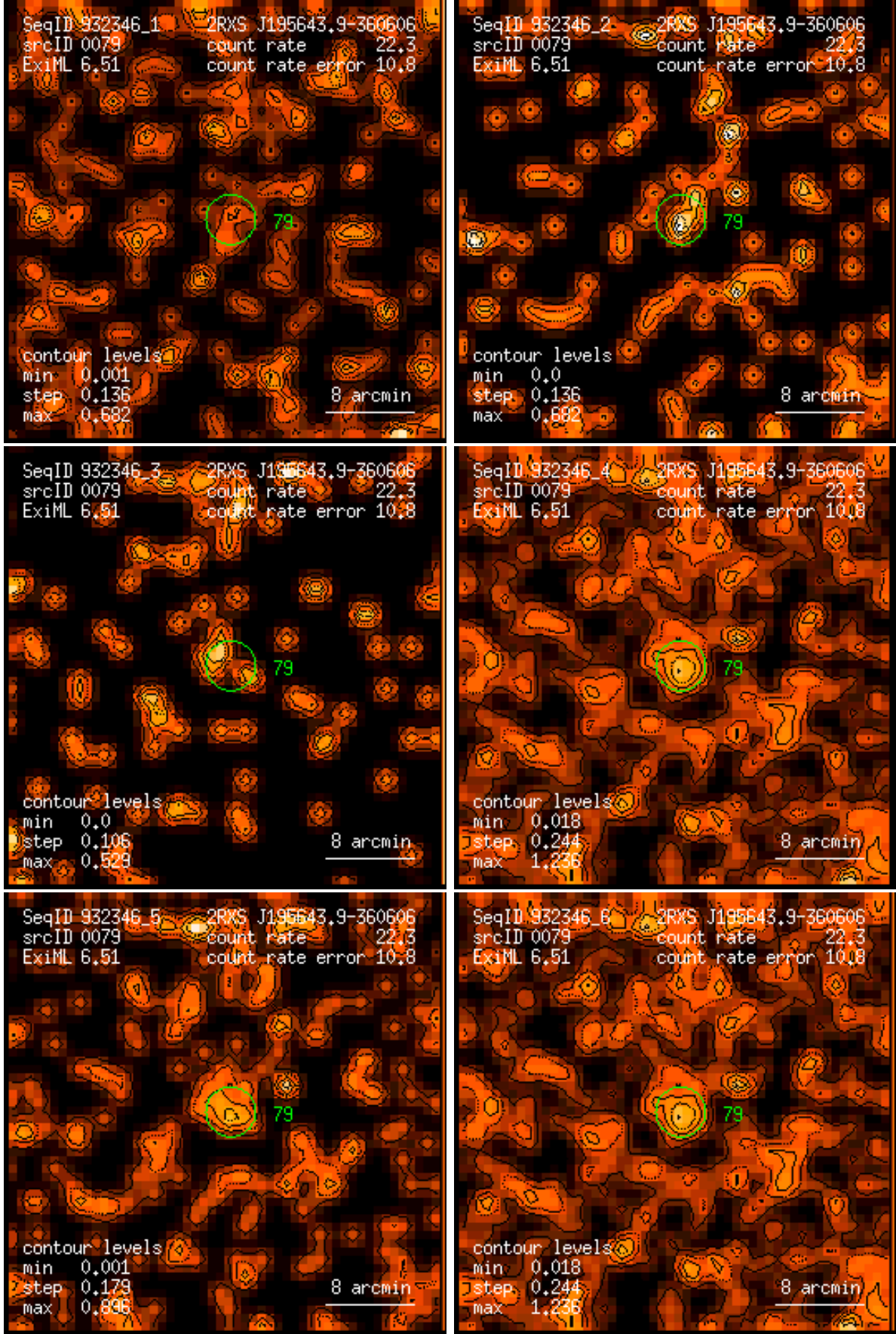
Figure 79: RASS 932346: detection 0079: band rate images, Gaussian filter: (1) PSPC channels 11 – 41, (2) 52 – 90, (3) 91 – 201, (4) 11 – 235, (5) 52 – 201, (6) 11 – 201. Broad band rates in counts/ks. Band rate contour levels in counts/ks/arcmin 2 .
