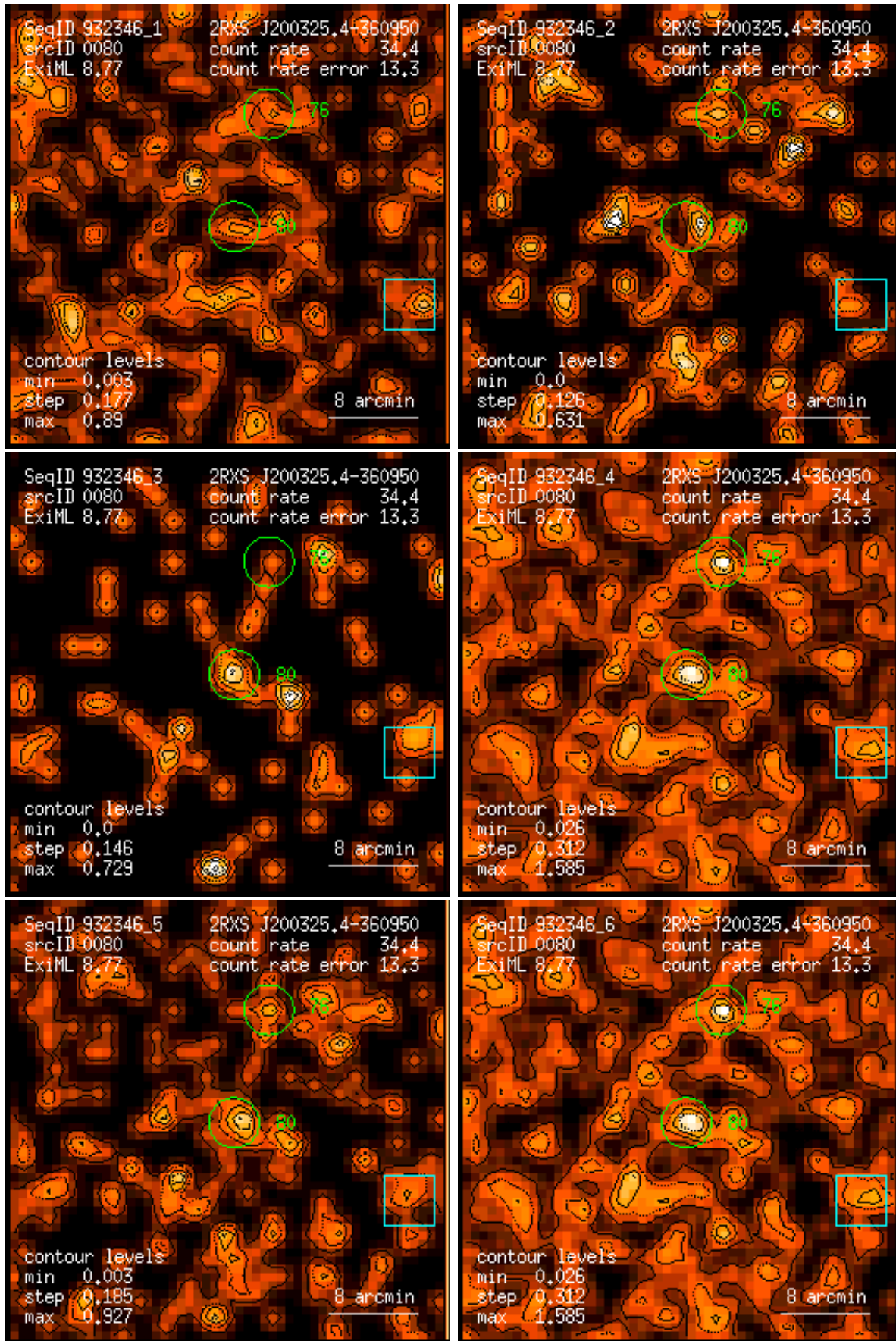
Figure 80: RASS 932346: detection 0080: band rate images, Gaussian filter: (1) PSPC channels 11 – 41, (2) 52 – 90, (3) 91 – 201, (4) 11 – 235, (5) 52 – 201, (6) 11 – 201. Broad band rates in counts/ks. Band rate contour levels in counts/ks/arcmin 2 .
