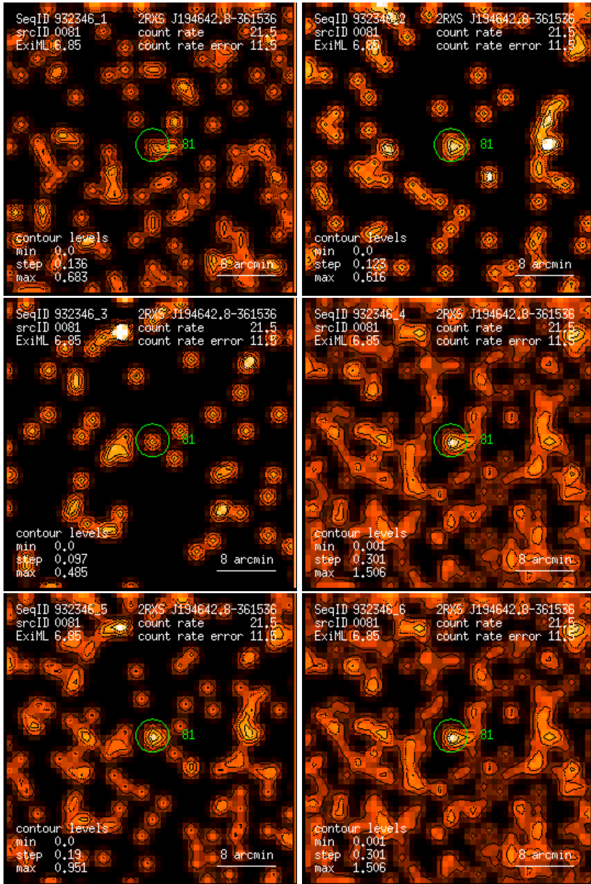
Figure 81: RASS 932346: detection 0081: band rate images, Gaussian filter: (1) PSPC channels 11 – 41, (2) 52 – 90, (3) 91 – 201, (4) 11 – 235, (5) 52 – 201, (6) 11 – 201. Broad band rates in counts/ks. Band rate contour levels in counts/ks/arcmin 2 .
