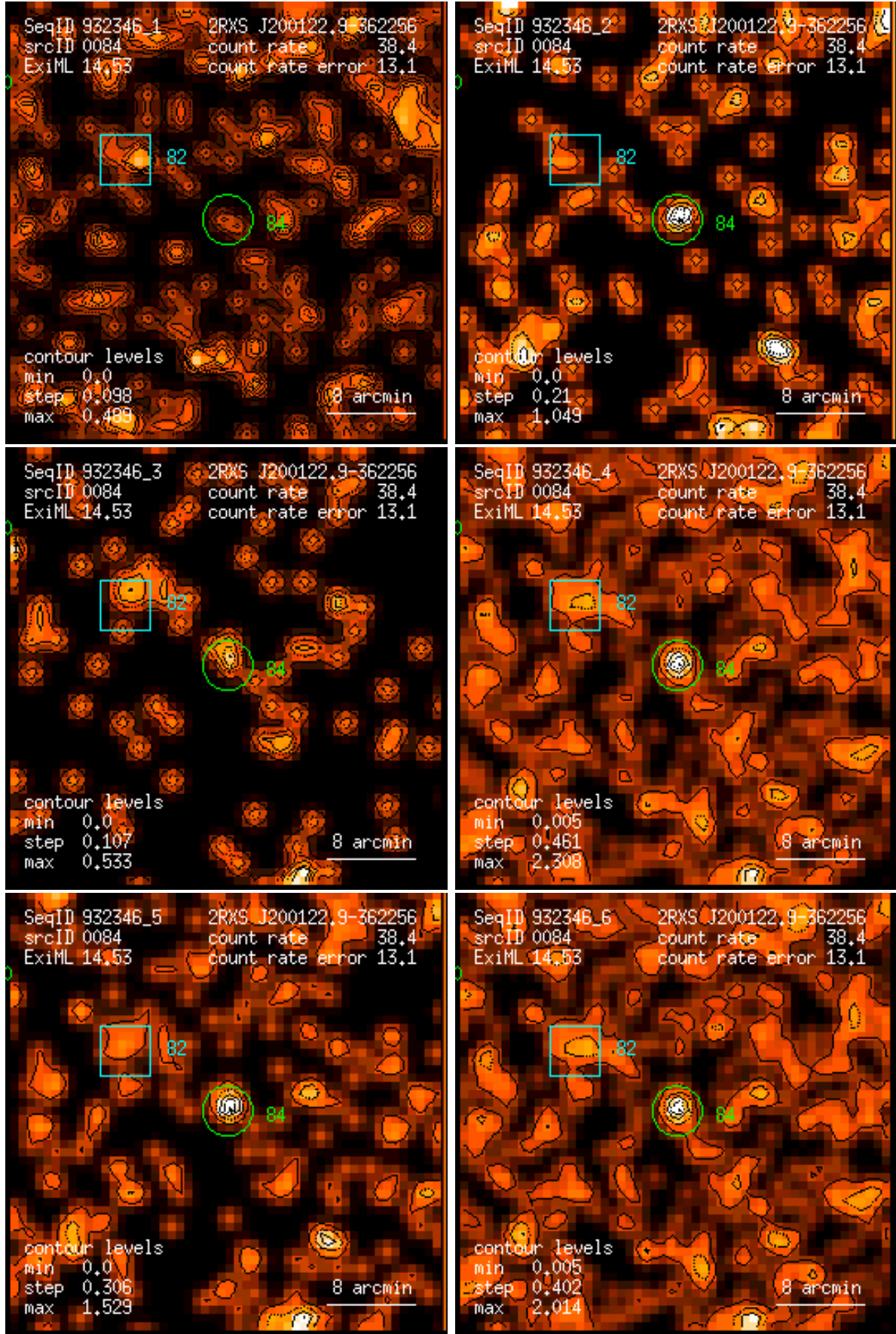
Figure 84: RASS 932346: detection 0084: band rate images, Gaussian filter: (1) PSPC channels 11 – 41, (2) 52 – 90, (3) 91 – 201, (4) 11 – 235, (5) 52 – 201, (6) 11 – 201. Broad band rates in counts/ks. Band rate contour levels in counts/ks/arcmin 2 .
