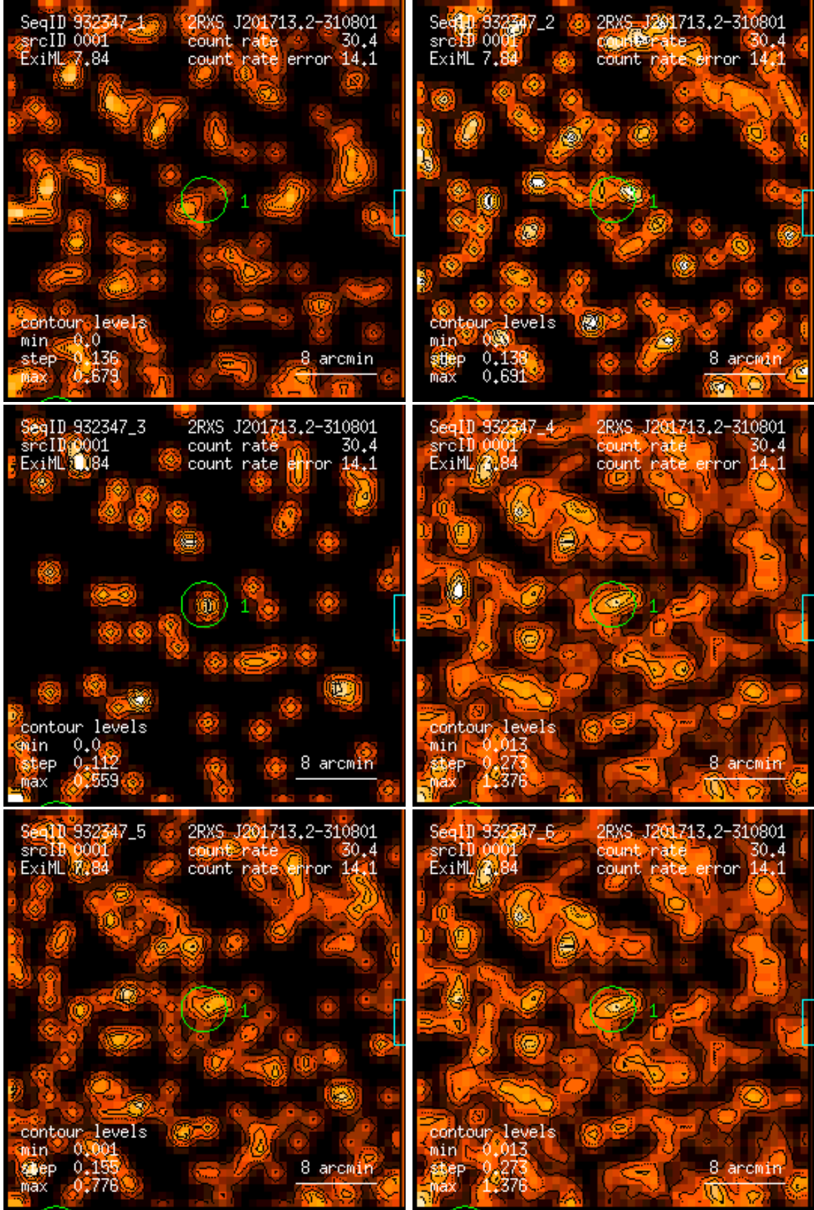
Figure 1: RASS 932347: detection 0001: band rate images, Gaussian filter: (1) PSPC channels 11 – 41, (2) 52 – 90, (3) 91 – 201, (4) 11 – 235, (5) 52 – 201, (6) 11 – 201. Broad band rates in counts/ks. Band rate contour levels in counts/ks/arcmin 2 .
