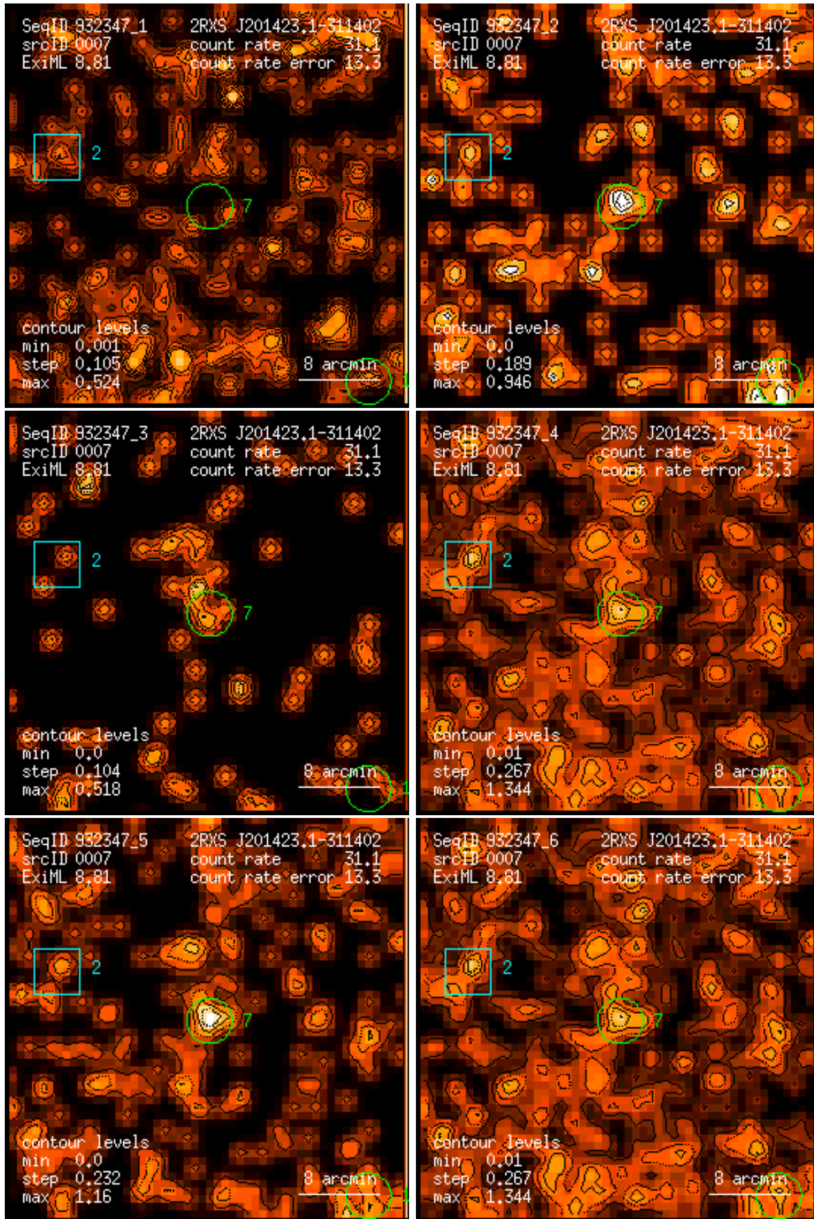
Figure 7: RASS 932347: detection 0007: band rate images, Gaussian filter: (1) PSPC channels 11 – 41, (2) 52 – 90, (3) 91 – 201, (4) 11 – 235, (5) 52 – 201, (6) 11 – 201. Broad band rates in counts/ks. Band rate contour levels in counts/ks/arcmin 2 .
