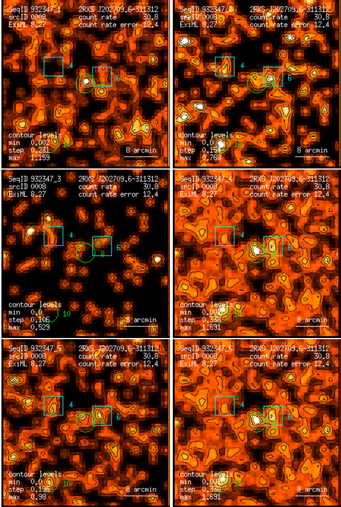
Figure 8: RASS 932347: detection 0008: band rate images, Gaussian filter: (1) PSPC channels 11 – 41, (2) 52 – 90, (3) 91 – 201, (4) 11 – 235, (5) 52 – 201, (6) 11 – 201. Broad band rates in counts/ks. Band rate contour levels in counts/ks/arcmin 2 .
