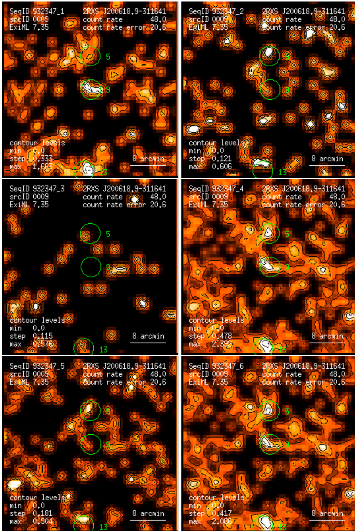
Figure 9: RASS 932347: detection 0009: band rate images, Gaussian filter: (1) PSPC channels 11 – 41, (2) 52 – 90, (3) 91 – 201, (4) 11 – 235, (5) 52 – 201, (6) 11 – 201. Broad band rates in counts/ks. Band rate contour levels in counts/ks/arcmin 2 .
