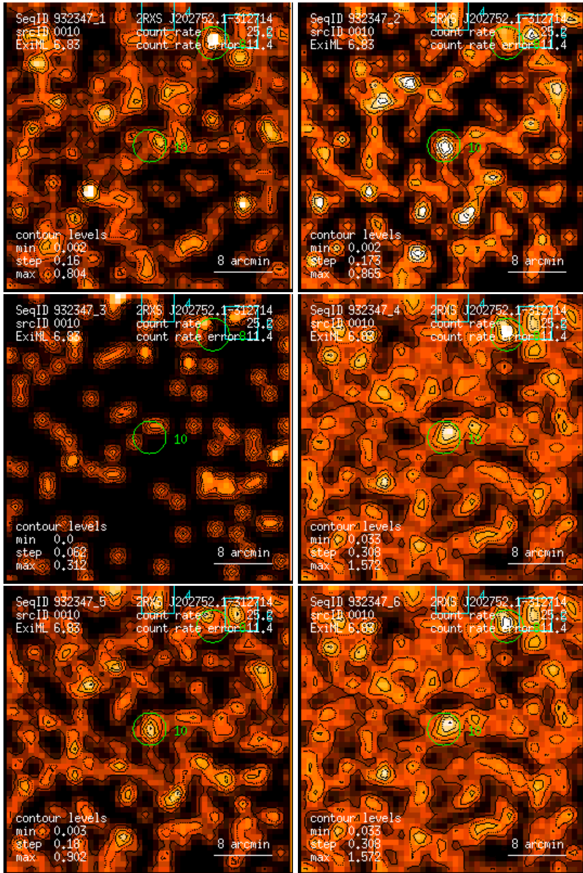
Figure 10: RASS 932347: detection 0010: band rate images, Gaussian filter: (1) PSPC channels 11 – 41, (2) 52 – 90, (3) 91 – 201, (4) 11 – 235, (5) 52 – 201, (6) 11 – 201. Broad band rates in counts/ks. Band rate contour levels in counts/ks/arcmin 2 .
