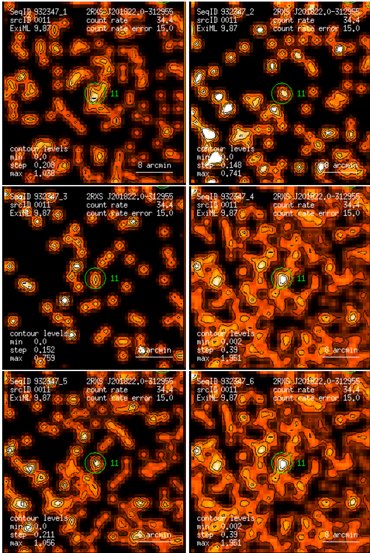
Figure 11: RASS 932347: detection 0011: band rate images, Gaussian filter: (1) PSPC channels 11 – 41, (2) 52 – 90, (3) 91 – 201, (4) 11 – 235, (5) 52 – 201, (6) 11 – 201. Broad band rates in counts/ks. Band rate contour levels in counts/ks/arcmin 2 .
