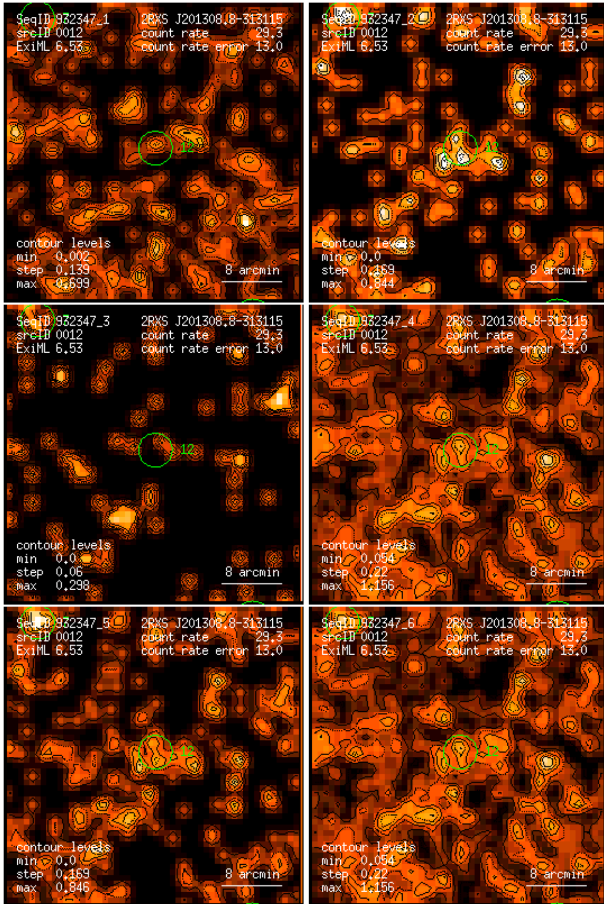
Figure 12: RASS 932347: detection 0012: band rate images, Gaussian filter: (1) PSPC channels 11 – 41, (2) 52 – 90, (3) 91 – 201, (4) 11 – 235, (5) 52 – 201, (6) 11 – 201. Broad band rates in counts/ks. Band rate contour levels in counts/ks/arcmin 2 .
