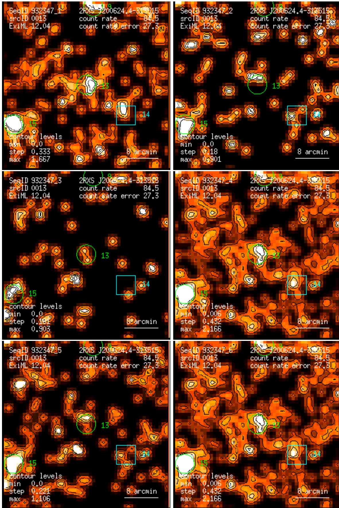
Figure 13: RASS 932347: detection 0013: band rate images, Gaussian filter: (1) PSPC channels 11 – 41, (2) 52 – 90, (3) 91 – 201, (4) 11 – 235, (5) 52 – 201, (6) 11 – 201. Broad band rates in counts/ks. Band rate contour levels in counts/ks/arcmin 2 .
