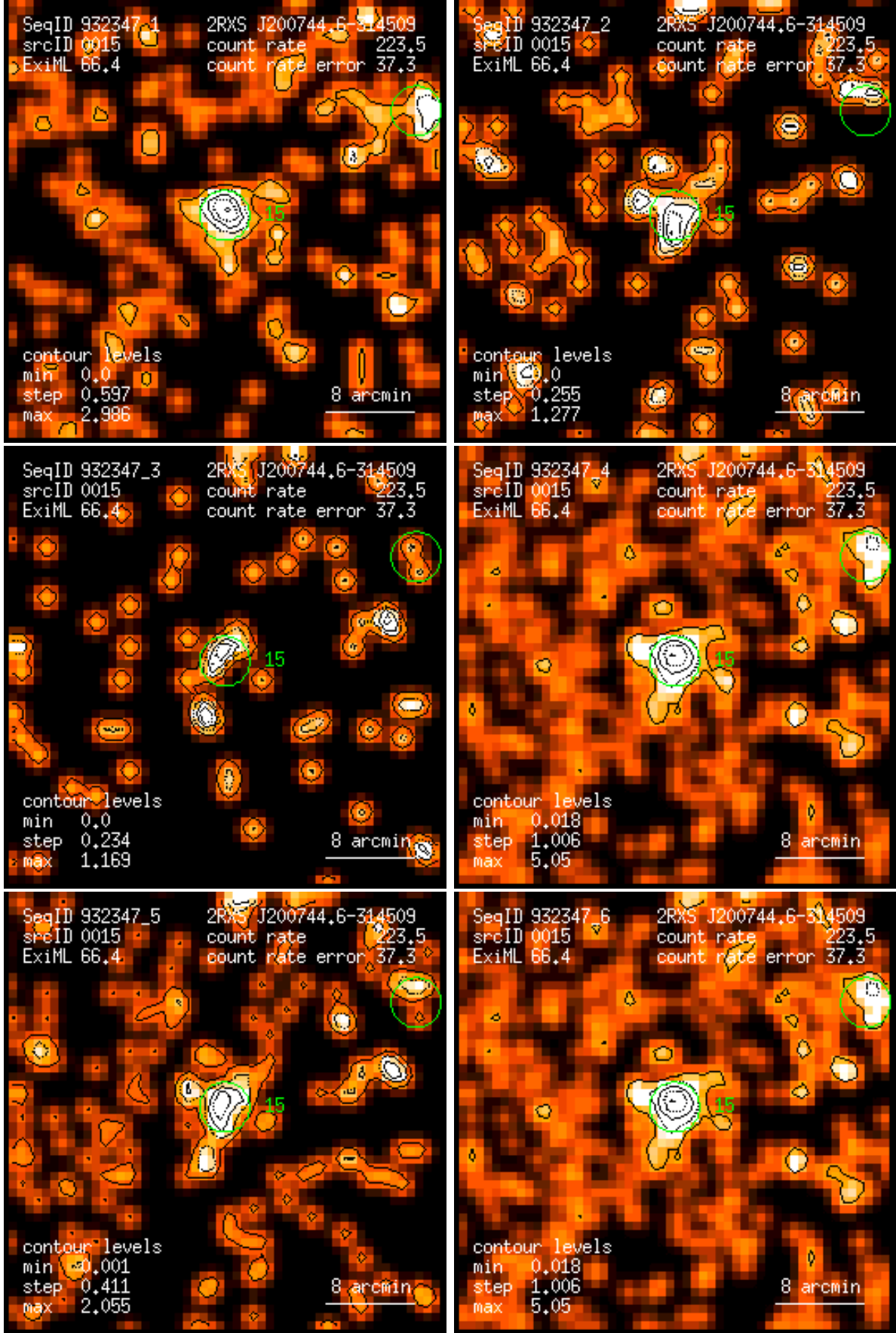
Figure 15: RASS 932347: detection 0015: band rate images, Gaussian filter: (1) PSPC channels 11 – 41, (2) 52 – 90, (3) 91 – 201, (4) 11 – 235, (5) 52 – 201, (6) 11 – 201. Broad band rates in counts/ks. Band rate contour levels in counts/ks/arcmin 2 .
