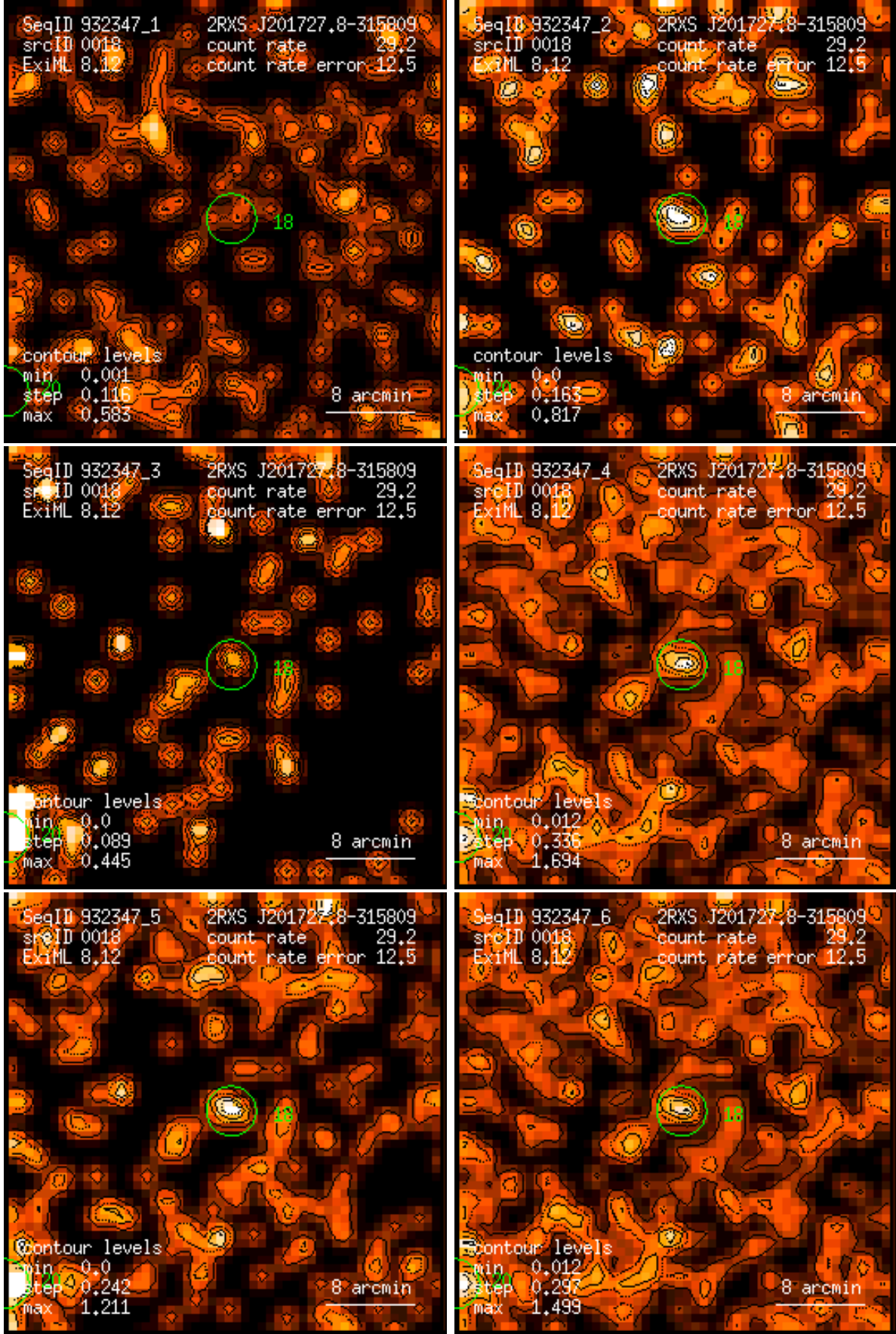
Figure 18: RASS 932347: detection 0018: band rate images, Gaussian filter: (1) PSPC channels 11 – 41, (2) 52 – 90, (3) 91 – 201, (4) 11 – 235, (5) 52 – 201, (6) 11 – 201. Broad band rates in counts/ks. Band rate contour levels in counts/ks/arcmin 2 .
