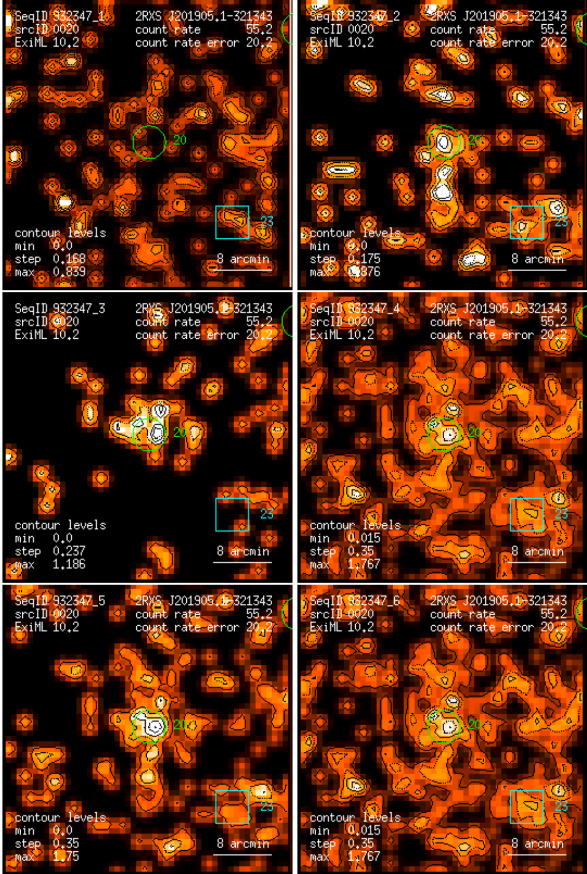
Figure 20: RASS 932347: detection 0020: band rate images, Gaussian filter: (1) PSPC channels 11 – 41, (2) 52 – 90, (3) 91 – 201, (4) 11 – 235, (5) 52 – 201, (6) 11 – 201. Broad band rates in counts/ks. Band rate contour levels in counts/ks/arcmin 2 .
