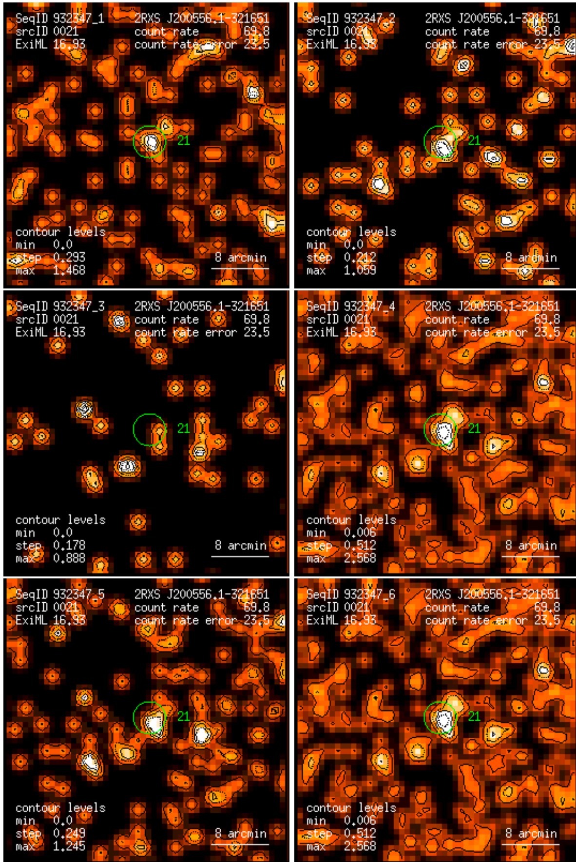
Figure 21: RASS 932347: detection 0021: band rate images, Gaussian filter: (1) PSPC channels 11 – 41, (2) 52 – 90, (3) 91 – 201, (4) 11 – 235, (5) 52 – 201, (6) 11 – 201. Broad band rates in counts/ks. Band rate contour levels in counts/ks/arcmin 2 .
