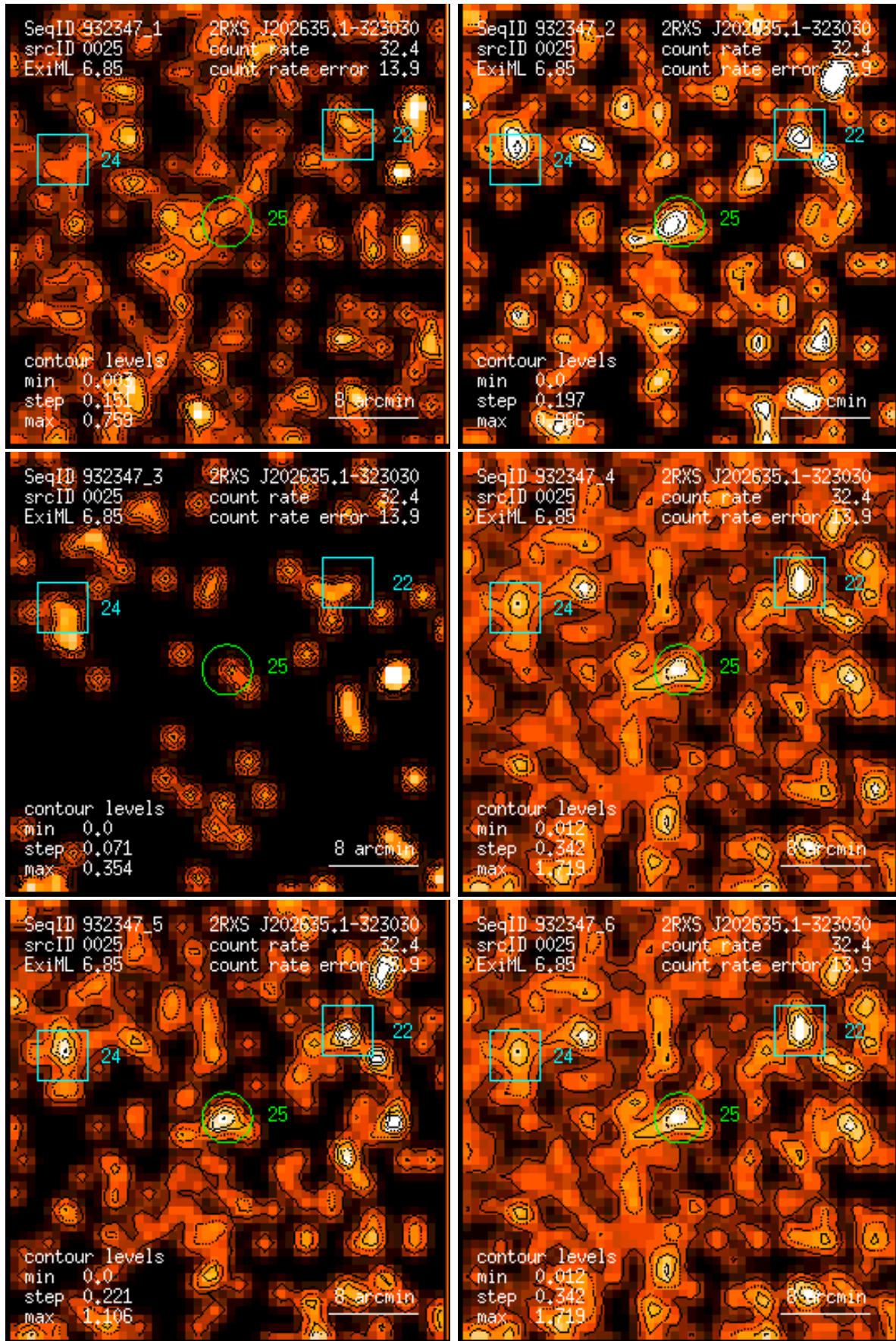
Figure 25: RASS 932347: detection 0025: band rate images, Gaussian filter: (1) PSPC channels 11 – 41, (2) 52 – 90, (3) 91 – 201, (4) 11 – 235, (5) 52 – 201, (6) 11 – 201. Broad band rates in counts/ks. Band rate contour levels in counts/ks/arcmin 2 .
