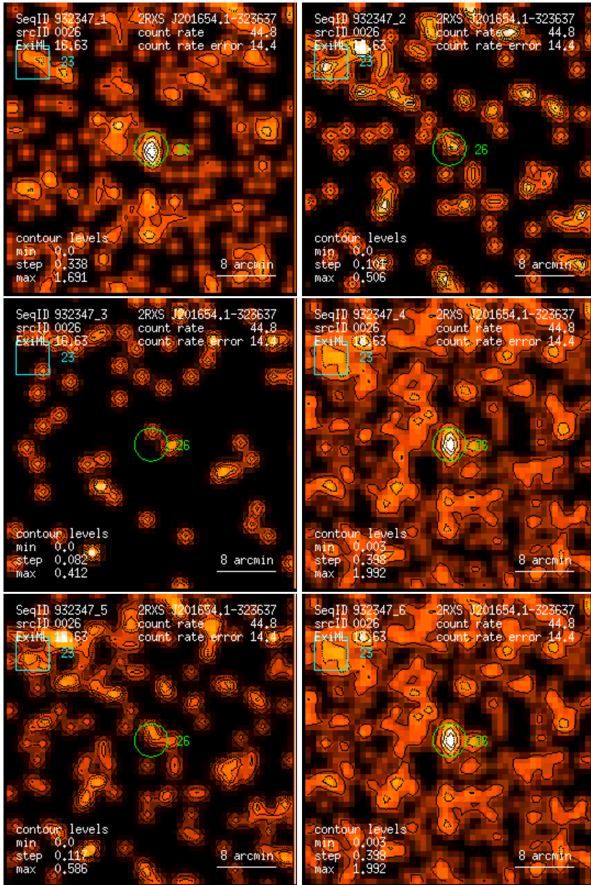
Figure 26: RASS 932347: detection 0026: band rate images, Gaussian filter: (1) PSPC channels 11 – 41, (2) 52 – 90, (3) 91 – 201, (4) 11 – 235, (5) 52 – 201, (6) 11 – 201. Broad band rates in counts/ks. Band rate contour levels in counts/ks/arcmin 2 .
