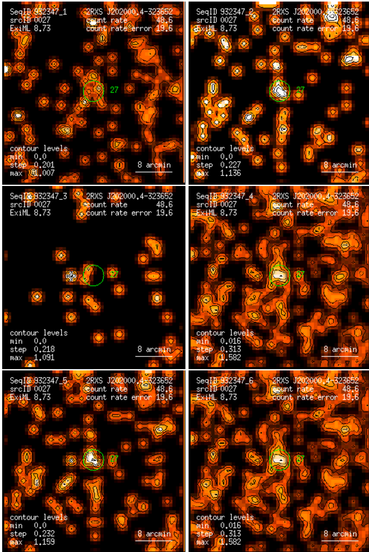
Figure 27: RASS 932347: detection 0027: band rate images, Gaussian filter: (1) PSPC channels 11 – 41, (2) 52 – 90, (3) 91 – 201, (4) 11 – 235, (5) 52 – 201, (6) 11 – 201. Broad band rates in counts/ks. Band rate contour levels in counts/ks/arcmin 2 .
