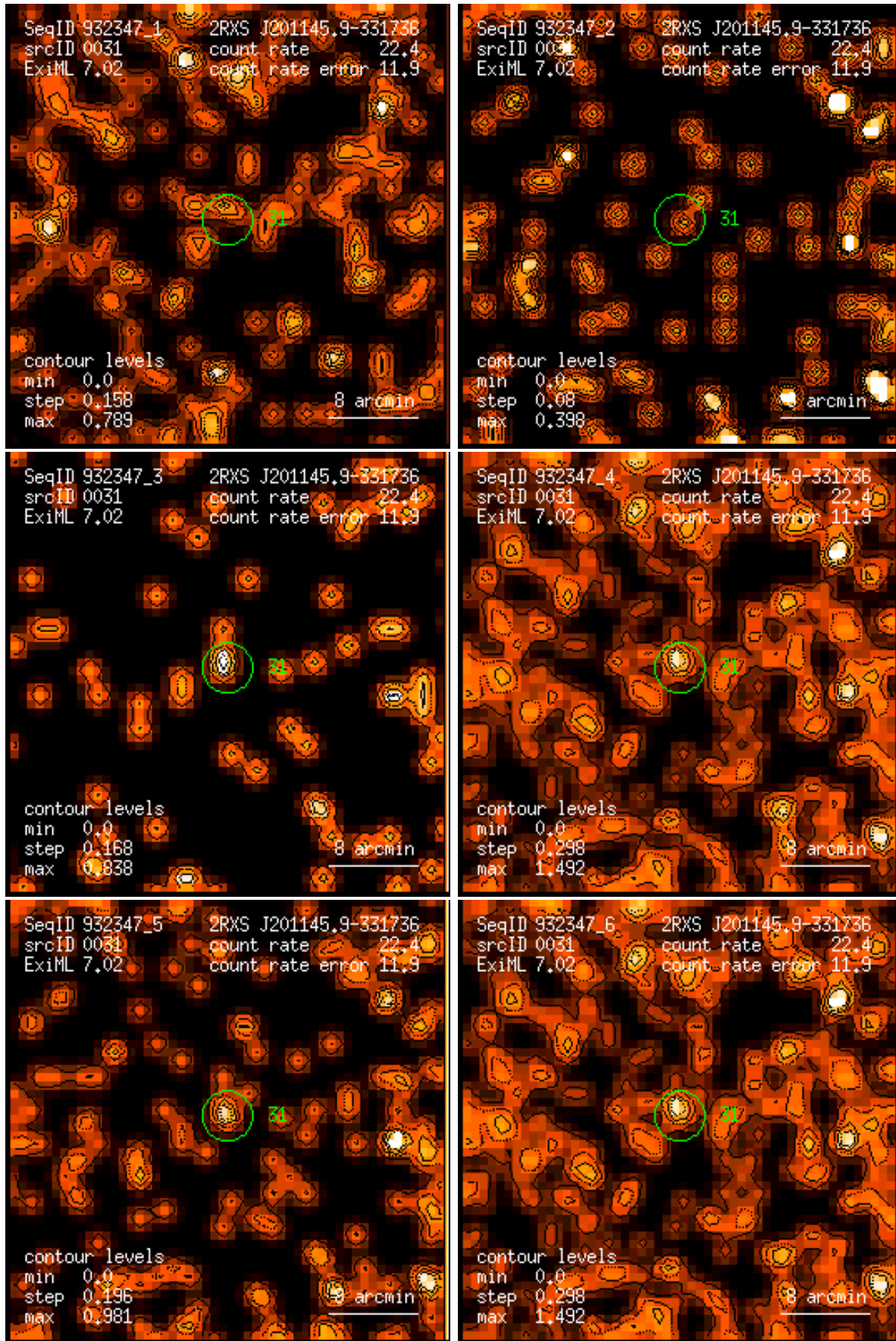
Figure 31: RASS 932347: detection 0031: band rate images, Gaussian filter: (1) PSPC channels 11 – 41, (2) 52 – 90, (3) 91 – 201, (4) 11 – 235, (5) 52 – 201, (6) 11 – 201. Broad band rates in counts/ks. Band rate contour levels in counts/ks/arcmin 2 .
