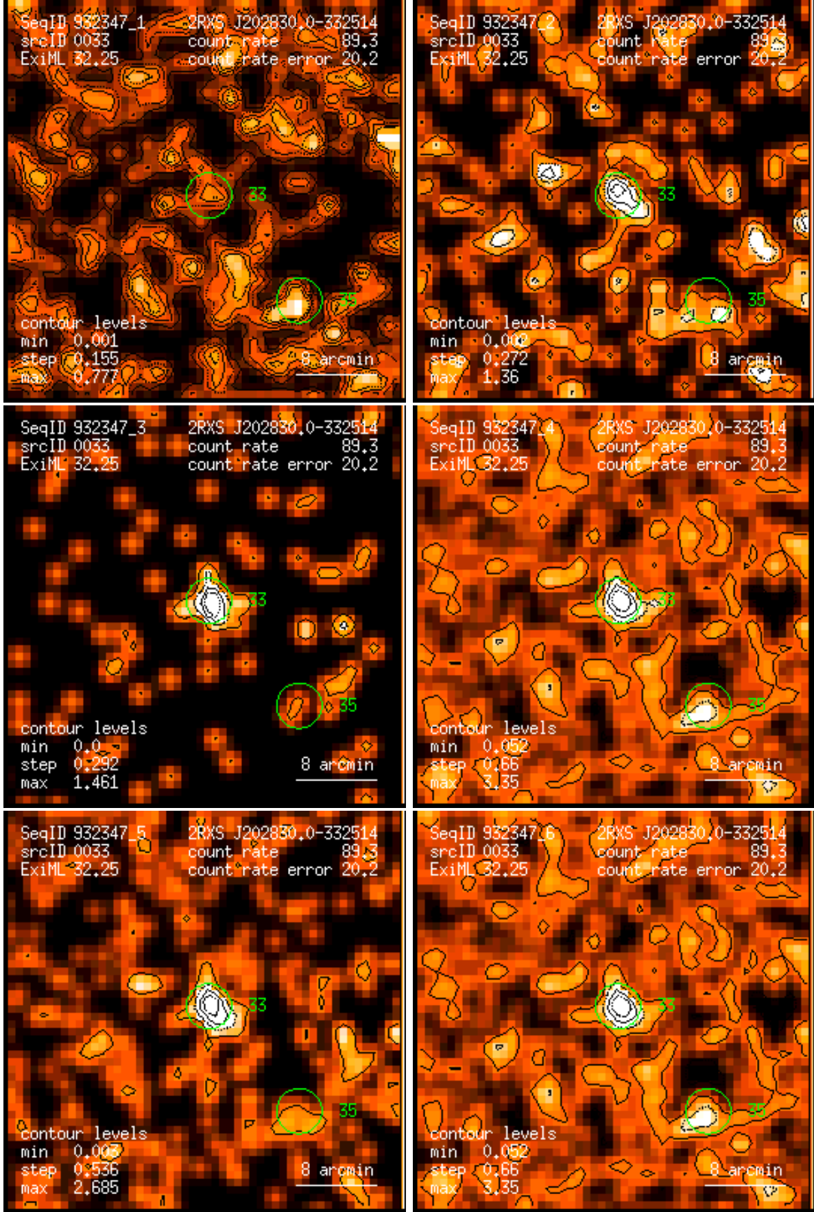
Figure 33: RASS 932347: detection 0033: band rate images, Gaussian filter: (1) PSPC channels 11 – 41, (2) 52 – 90, (3) 91 – 201, (4) 11 – 235, (5) 52 – 201, (6) 11 – 201. Broad band rates in counts/ks. Band rate contour levels in counts/ks/arcmin 2 .
