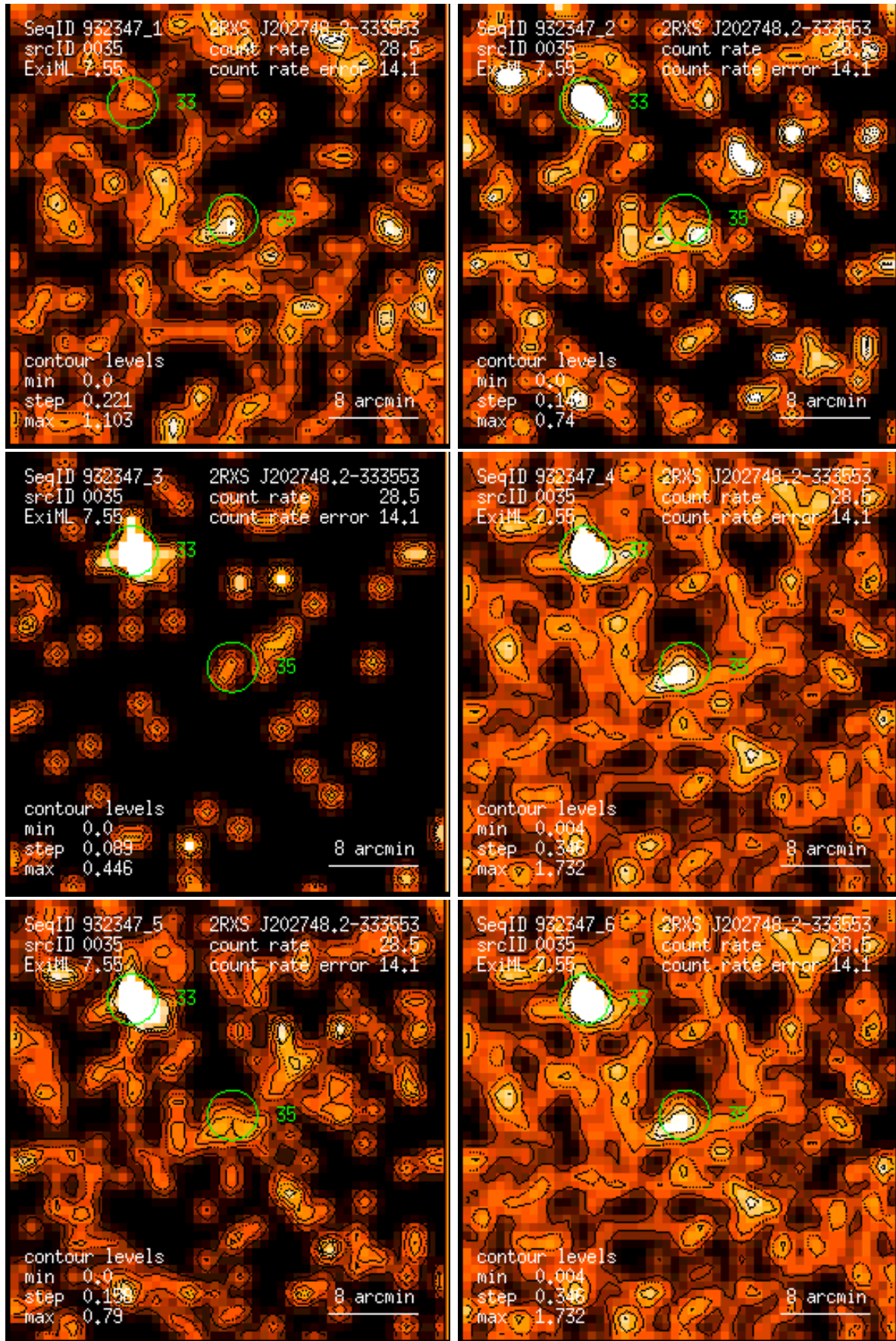
Figure 35: RASS 932347: detection 0035: band rate images, Gaussian filter: (1) PSPC channels 11 – 41, (2) 52 – 90, (3) 91 – 201, (4) 11 – 235, (5) 52 – 201, (6) 11 – 201. Broad band rates in counts/ks. Band rate contour levels in counts/ks/arcmin 2 .
