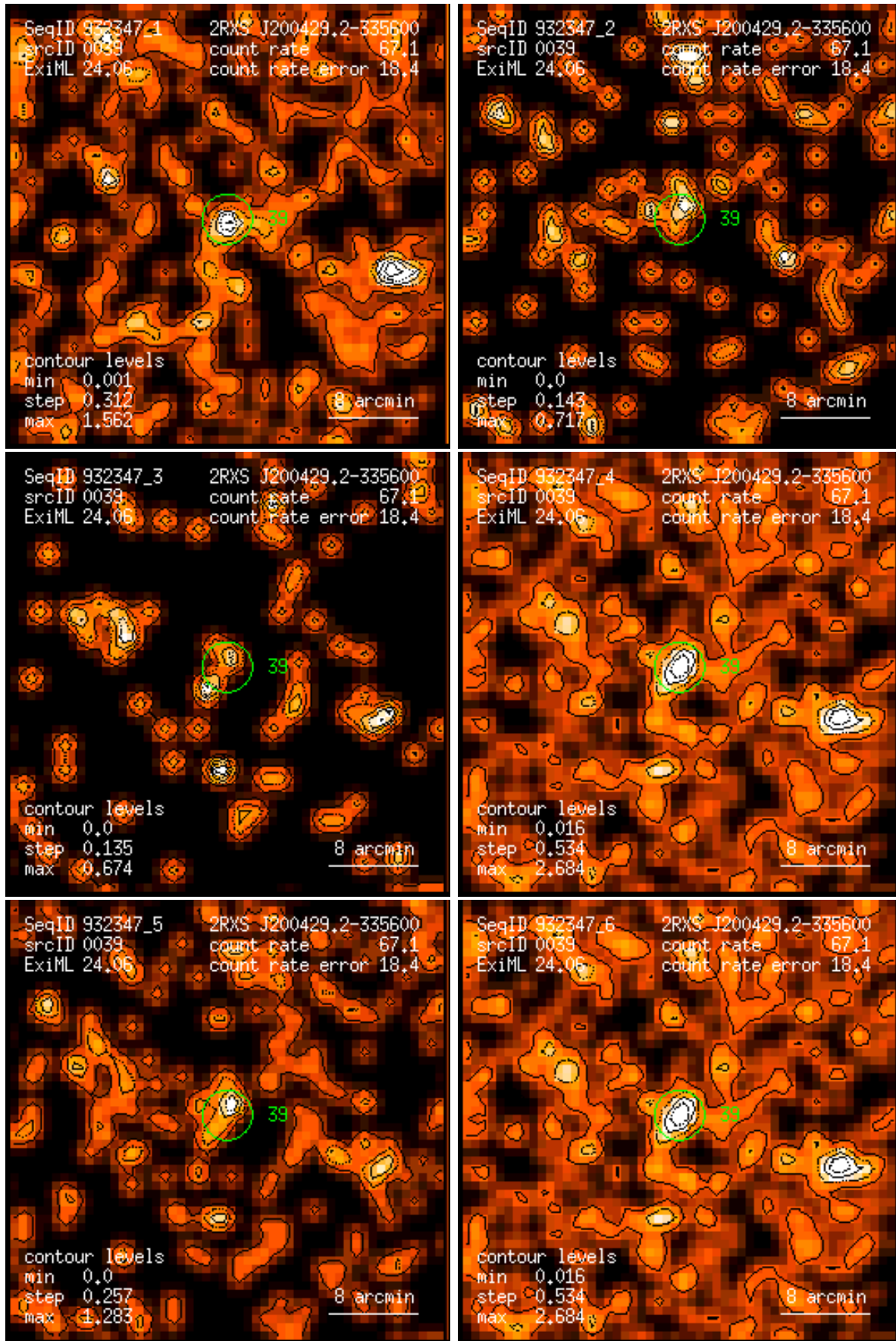
Figure 39: RASS 932347: detection 0039: band rate images, Gaussian filter: (1) PSPC channels 11 – 41, (2) 52 – 90, (3) 91 – 201, (4) 11 – 235, (5) 52 – 201, (6) 11 – 201. Broad band rates in counts/ks. Band rate contour levels in counts/ks/arcmin 2 .
