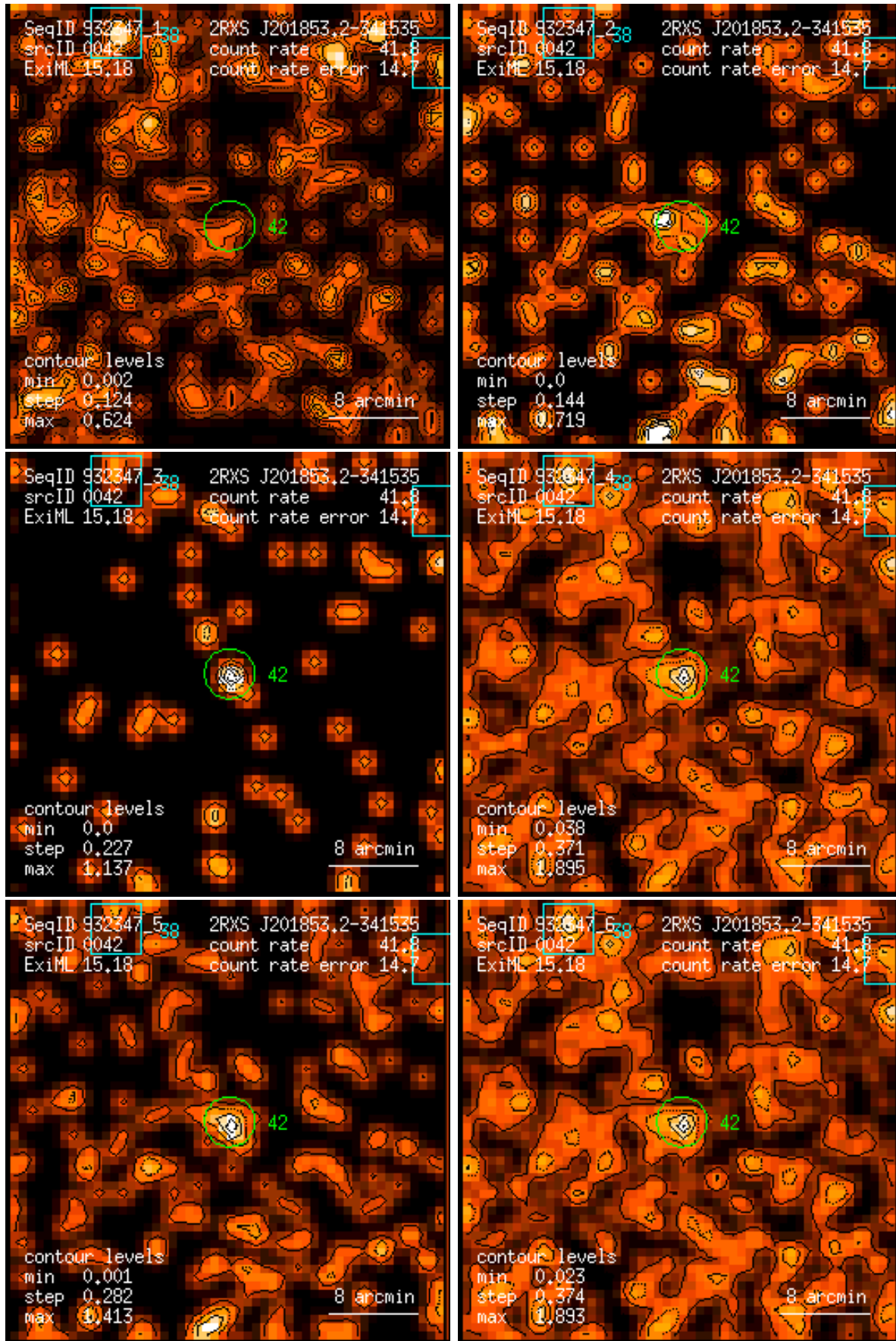
Figure 42: RASS 932347: detection 0042: band rate images, Gaussian filter: (1) PSPC channels 11 – 41, (2) 52 – 90, (3) 91 – 201, (4) 11 – 235, (5) 52 – 201, (6) 11 – 201. Broad band rates in counts/ks. Band rate contour levels in counts/ks/arcmin 2 .
