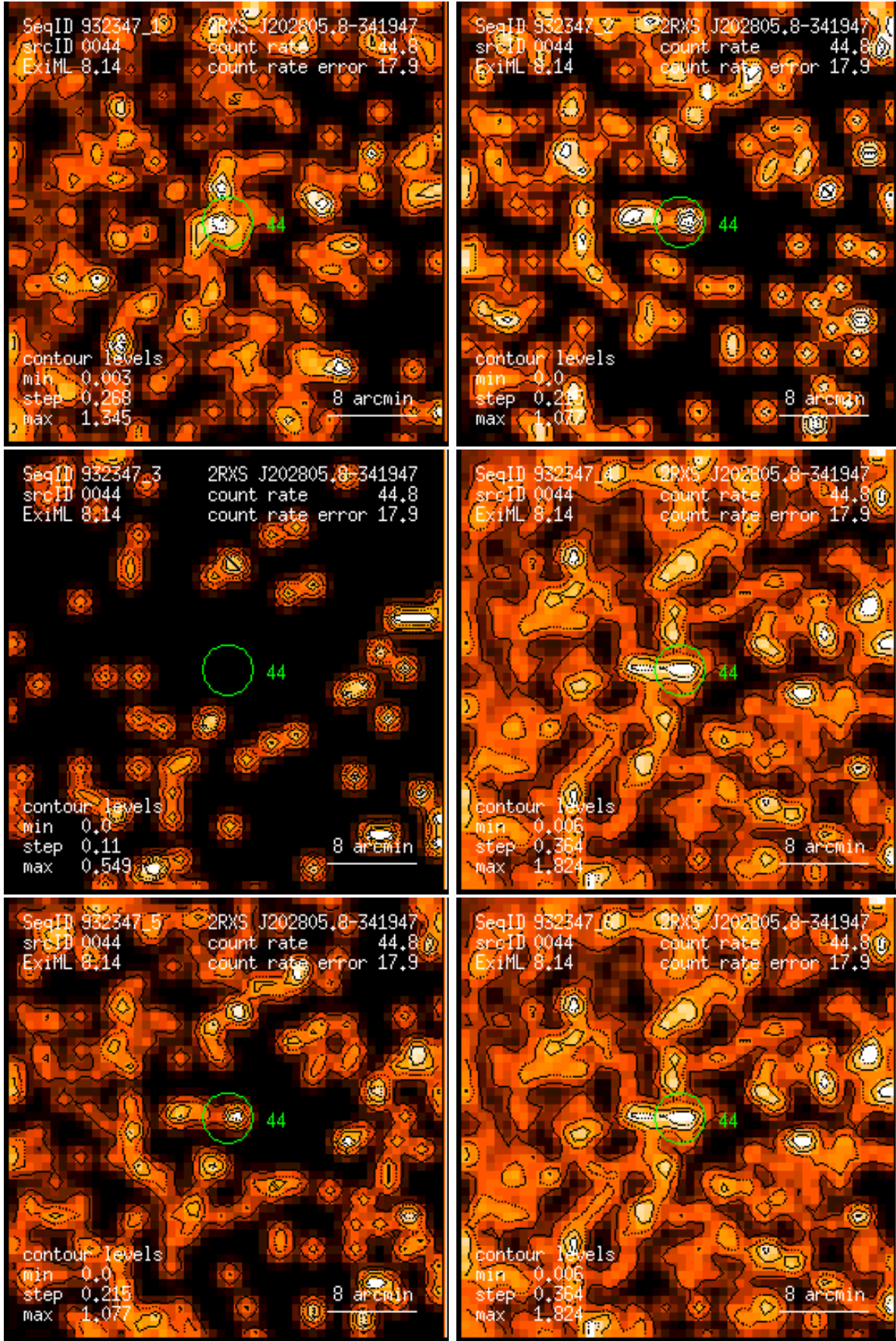
Figure 44: RASS 932347: detection 0044: band rate images, Gaussian filter: (1) PSPC channels 11 – 41, (2) 52 – 90, (3) 91 – 201, (4) 11 – 235, (5) 52 – 201, (6) 11 – 201. Broad band rates in counts/ks. Band rate contour levels in counts/ks/arcmin 2 .
