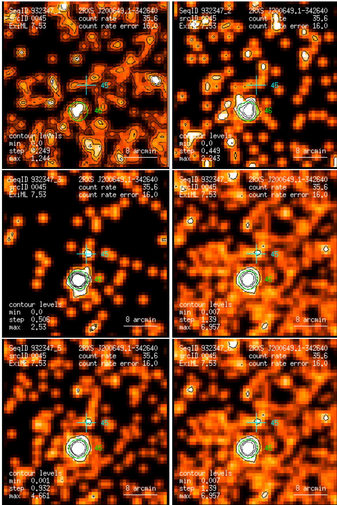
Figure 45: RASS 932347: detection 0045: band rate images, Gaussian filter: (1) PSPC channels 11 – 41, (2) 52 – 90, (3) 91 – 201, (4) 11 – 235, (5) 52 – 201, (6) 11 – 201. Broad band rates in counts/ks. Band rate contour levels in counts/ks/arcmin 2 .
