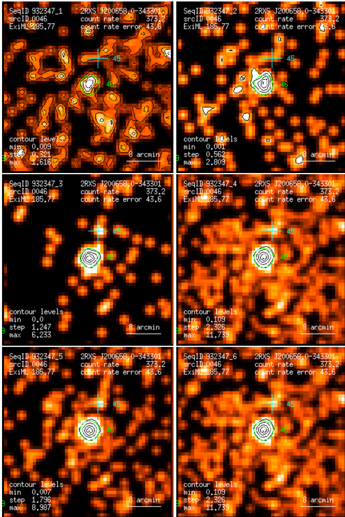
Figure 46: RASS 932347: detection 0046: band rate images, Gaussian filter: (1) PSPC channels 11 – 41, (2) 52 – 90, (3) 91 – 201, (4) 11 – 235, (5) 52 – 201, (6) 11 – 201. Broad band rates in counts/ks. Band rate contour levels in counts/ks/arcmin 2 .
