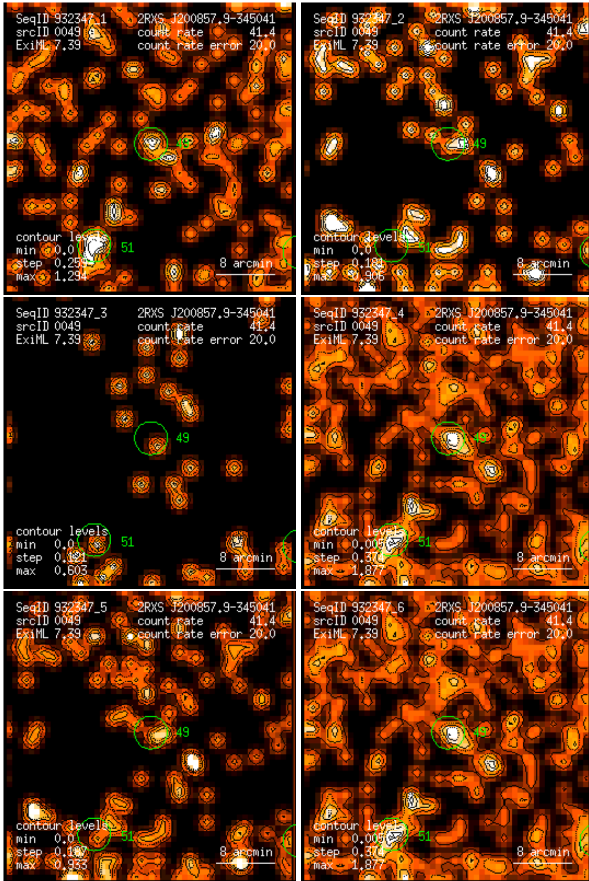
Figure 49: RASS 932347: detection 0049: band rate images, Gaussian filter: (1) PSPC channels 11 – 41, (2) 52 – 90, (3) 91 – 201, (4) 11 – 235, (5) 52 – 201, (6) 11 – 201. Broad band rates in counts/ks. Band rate contour levels in counts/ks/arcmin 2 .
