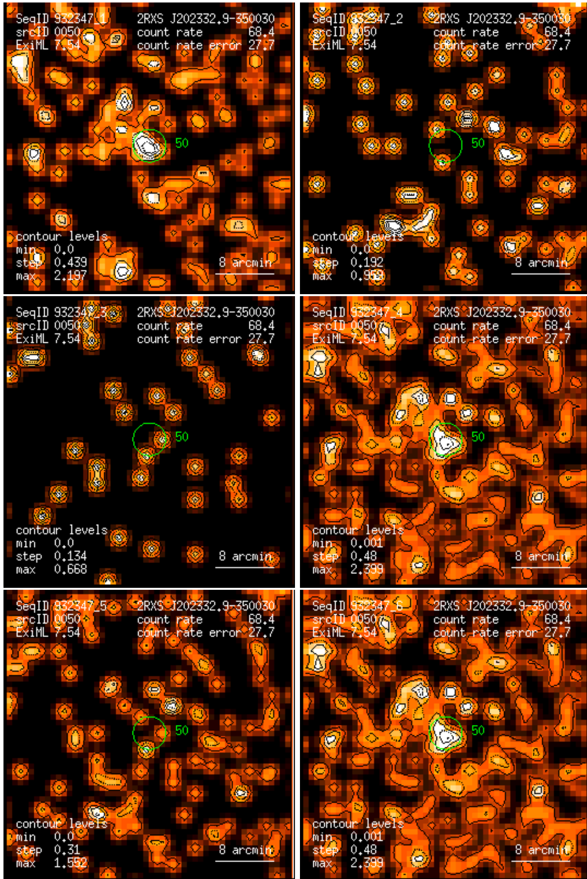
Figure 50: RASS 932347: detection 0050: band rate images, Gaussian filter: (1) PSPC channels 11 – 41, (2) 52 – 90, (3) 91 – 201, (4) 11 – 235, (5) 52 – 201, (6) 11 – 201. Broad band rates in counts/ks. Band rate contour levels in counts/ks/arcmin 2 .
