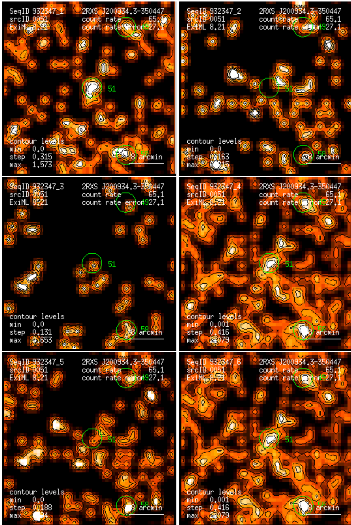
Figure 51: RASS 932347: detection 0051: band rate images, Gaussian filter: (1) PSPC channels 11 – 41, (2) 52 – 90, (3) 91 – 201, (4) 11 – 235, (5) 52 – 201, (6) 11 – 201. Broad band rates in counts/ks. Band rate contour levels in counts/ks/arcmin 2 .
